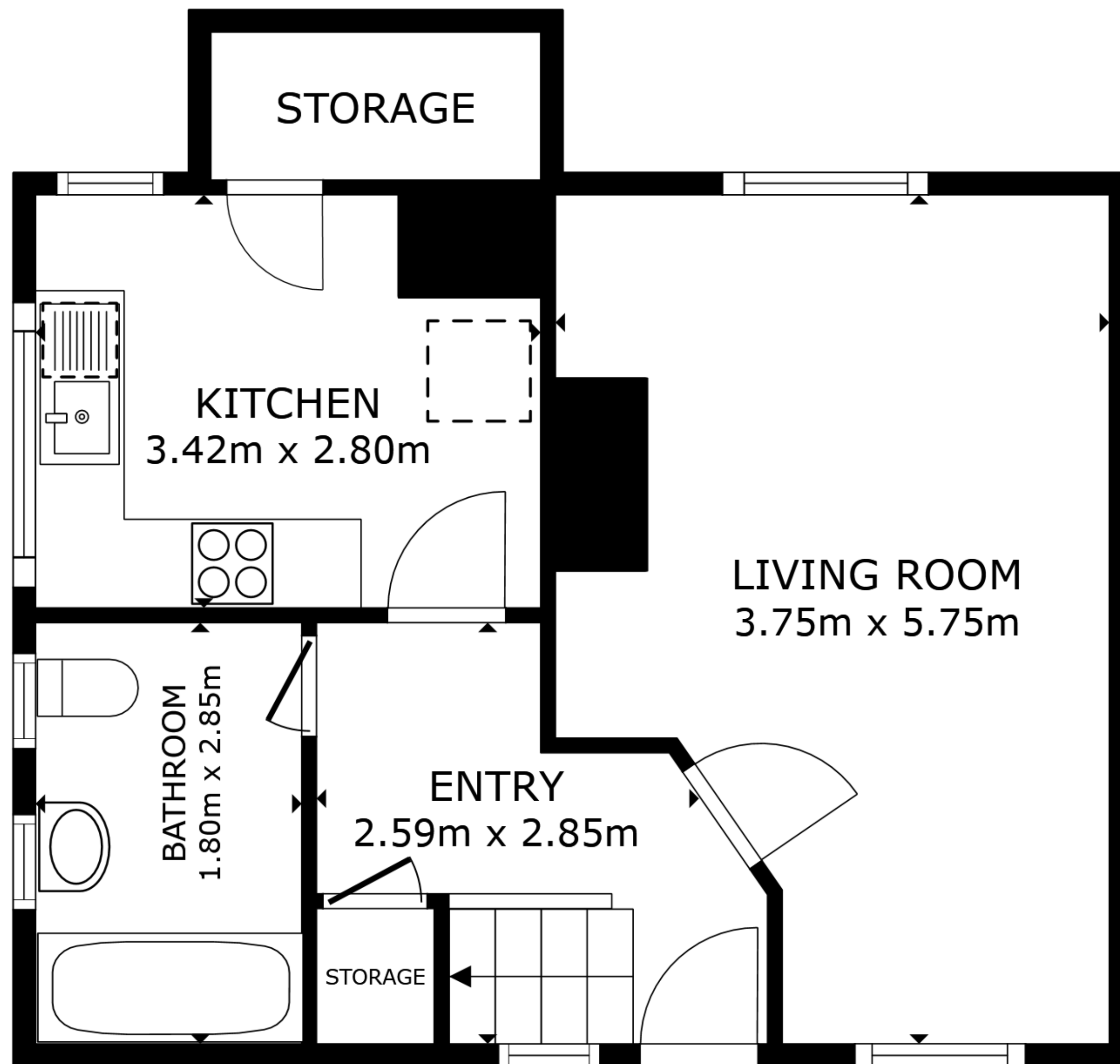
FLOOR 1
