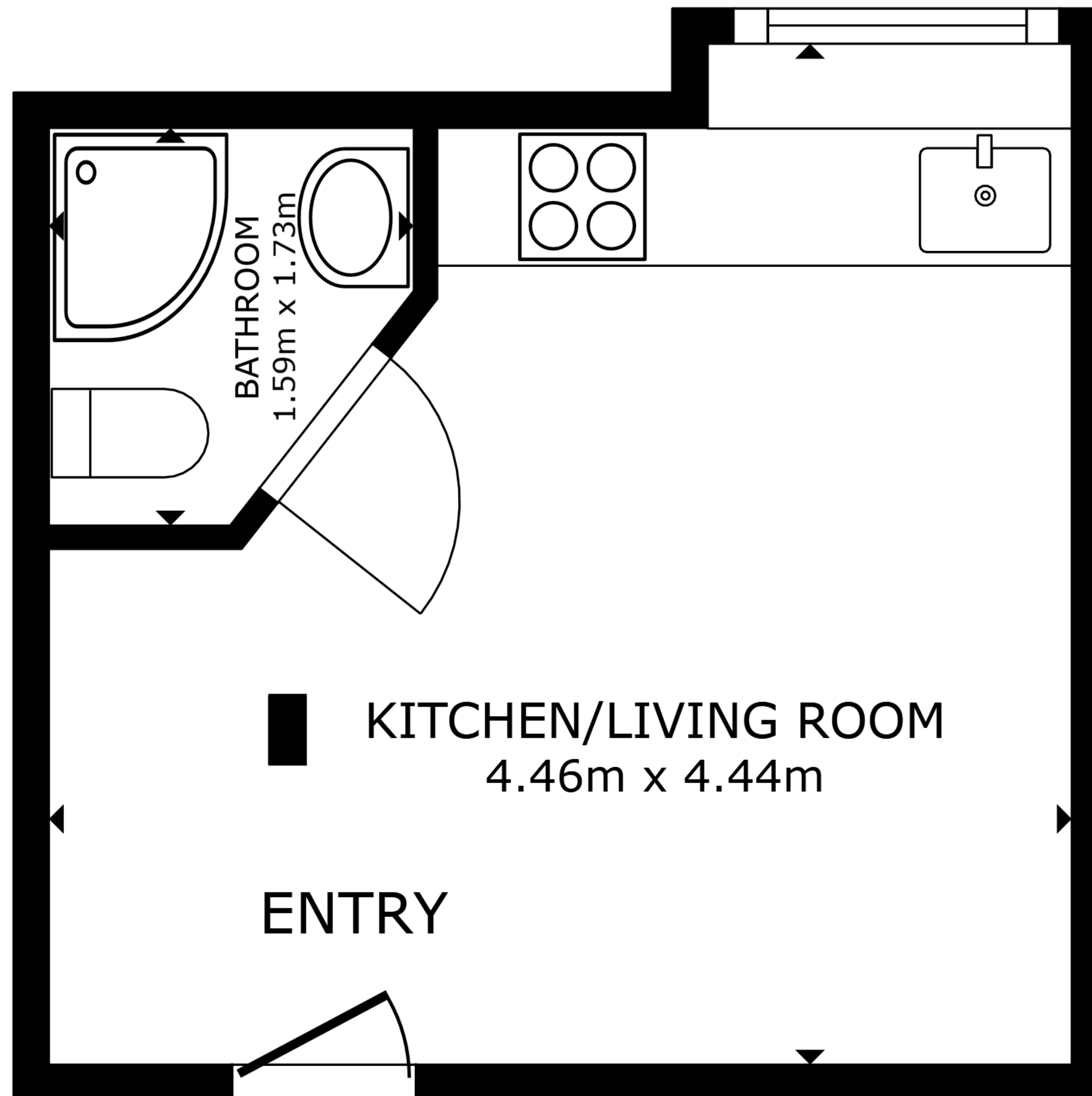
FLOOR PLAN
