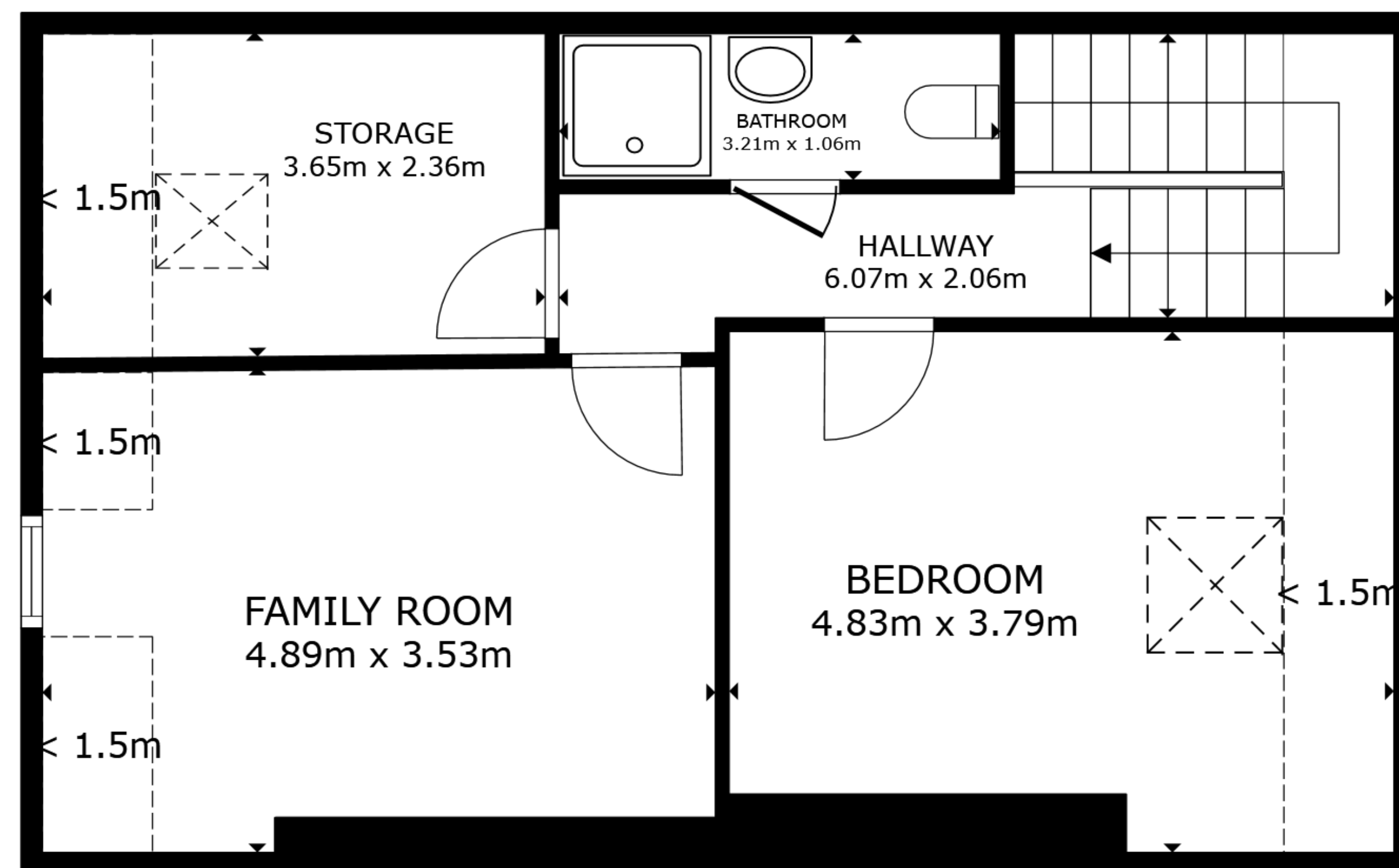
FLOOR 2
