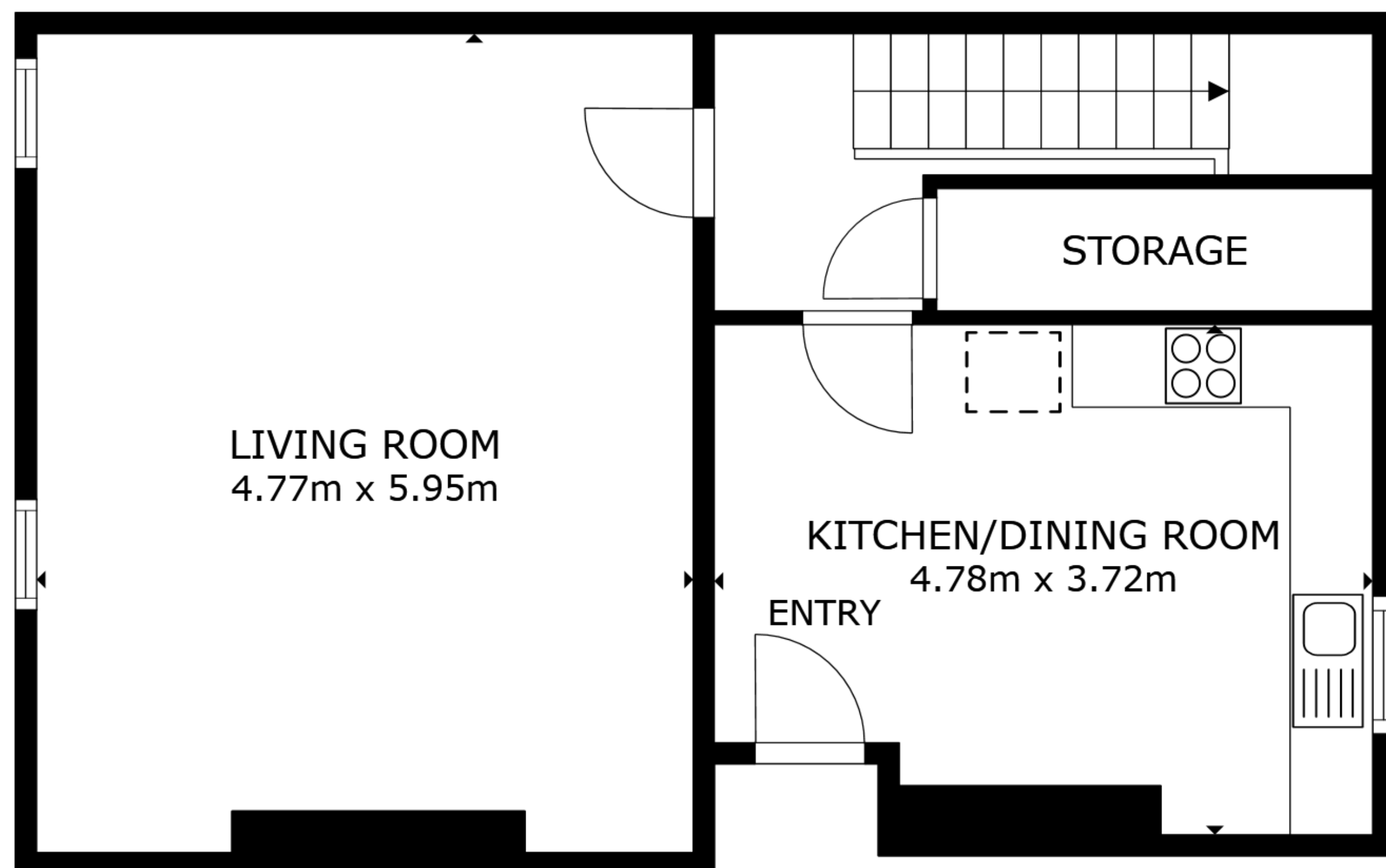
FLOOR 1
