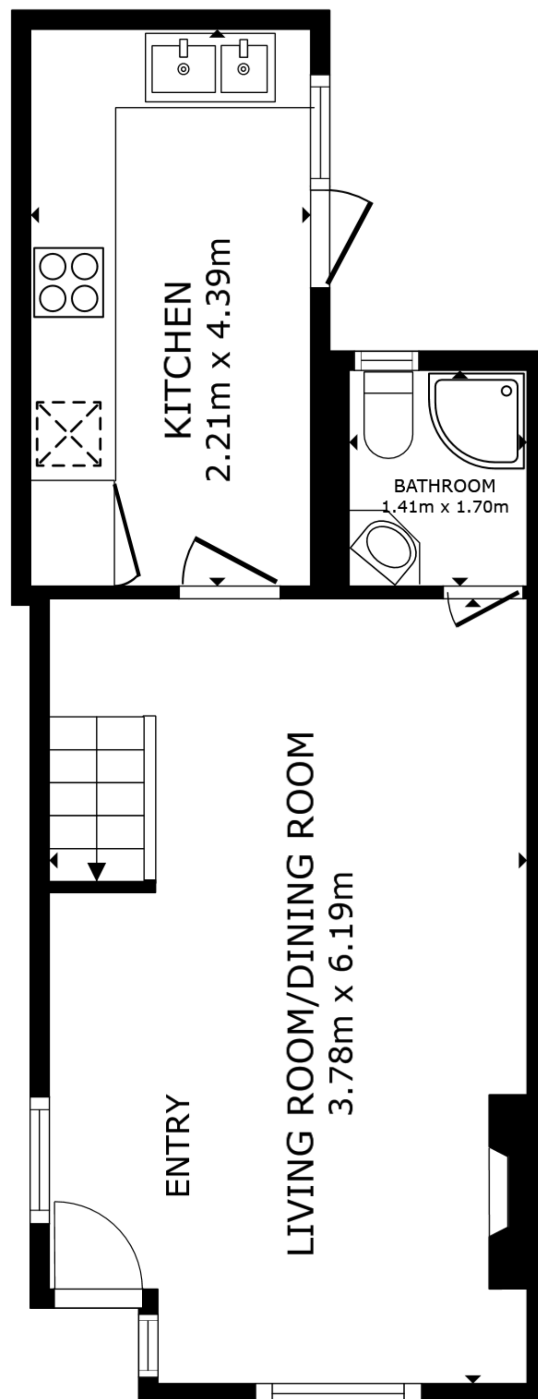
FLOOR 1
