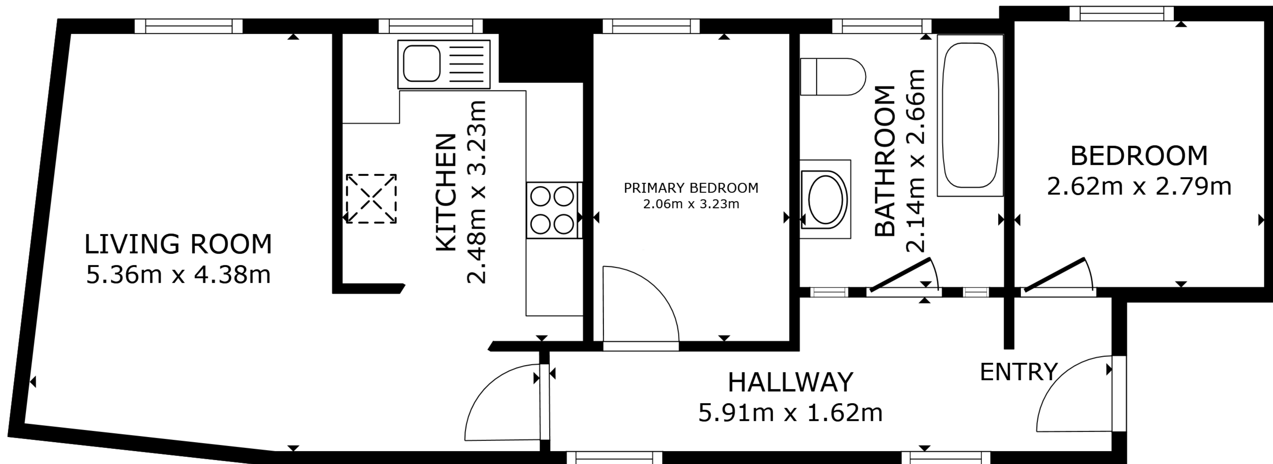
FLOOR PLAN
