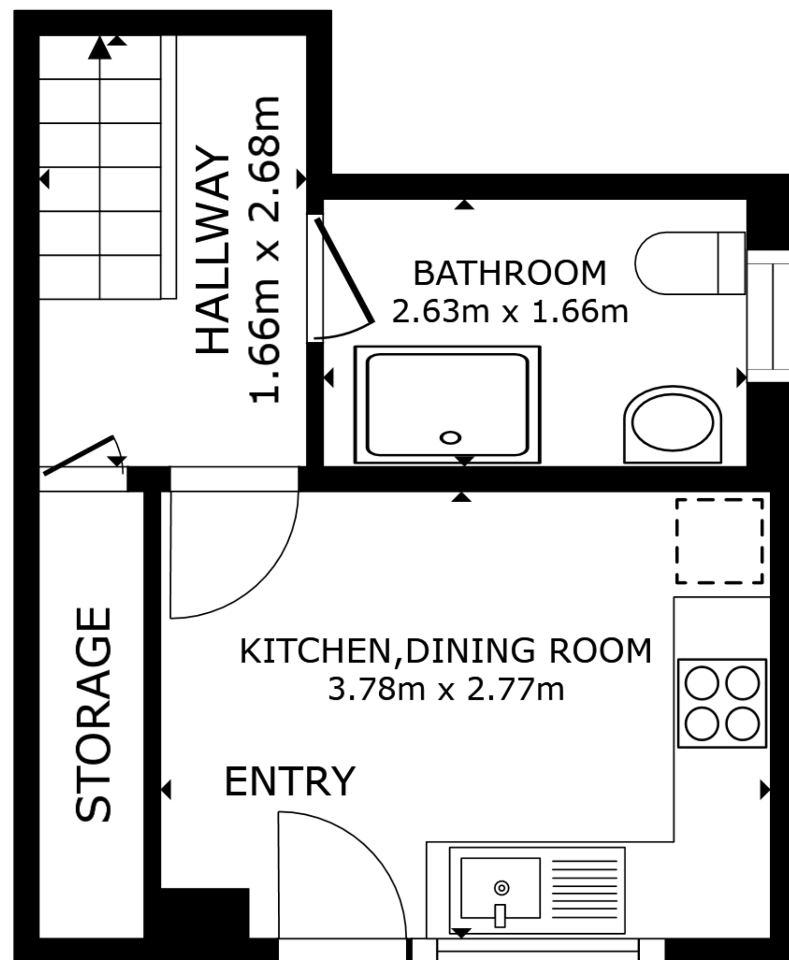
FLOOR 1
