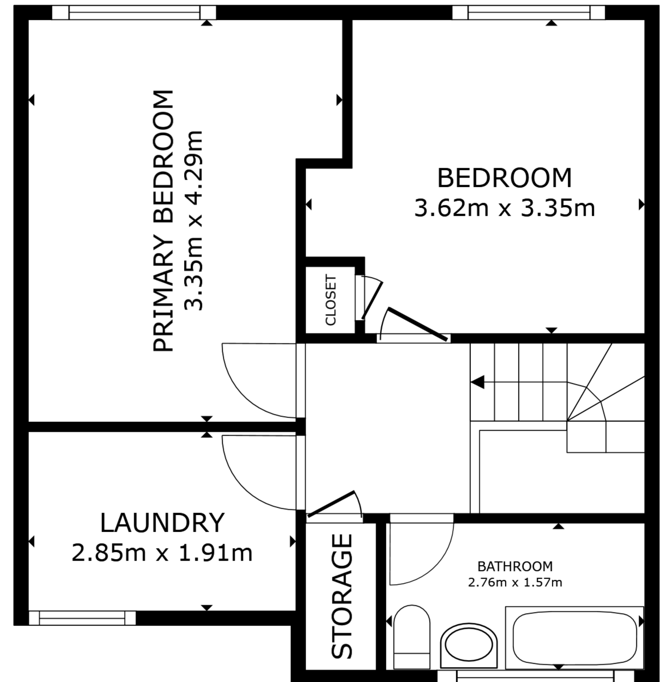
FLOOR 2
