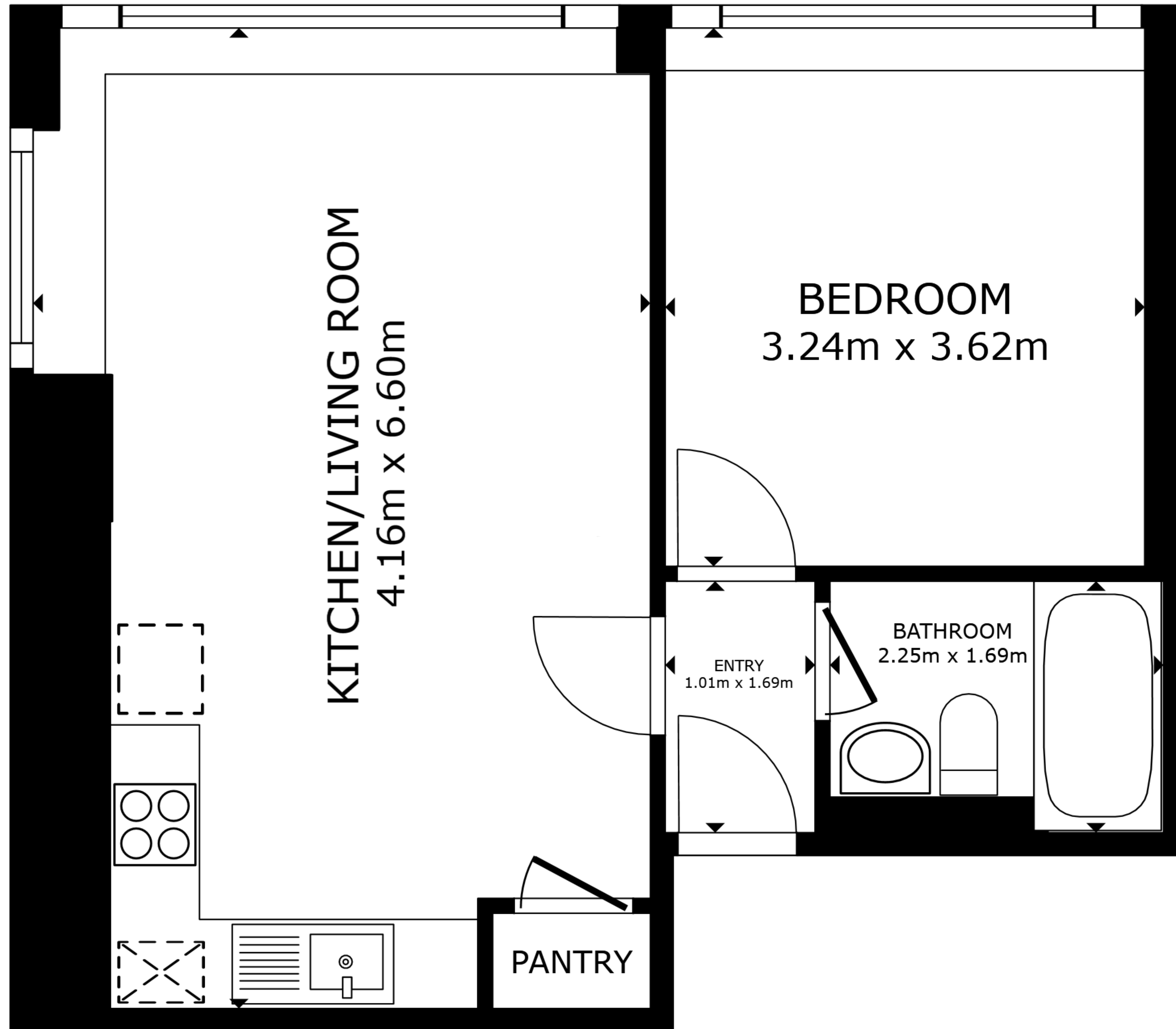
FLOOR PLAN
