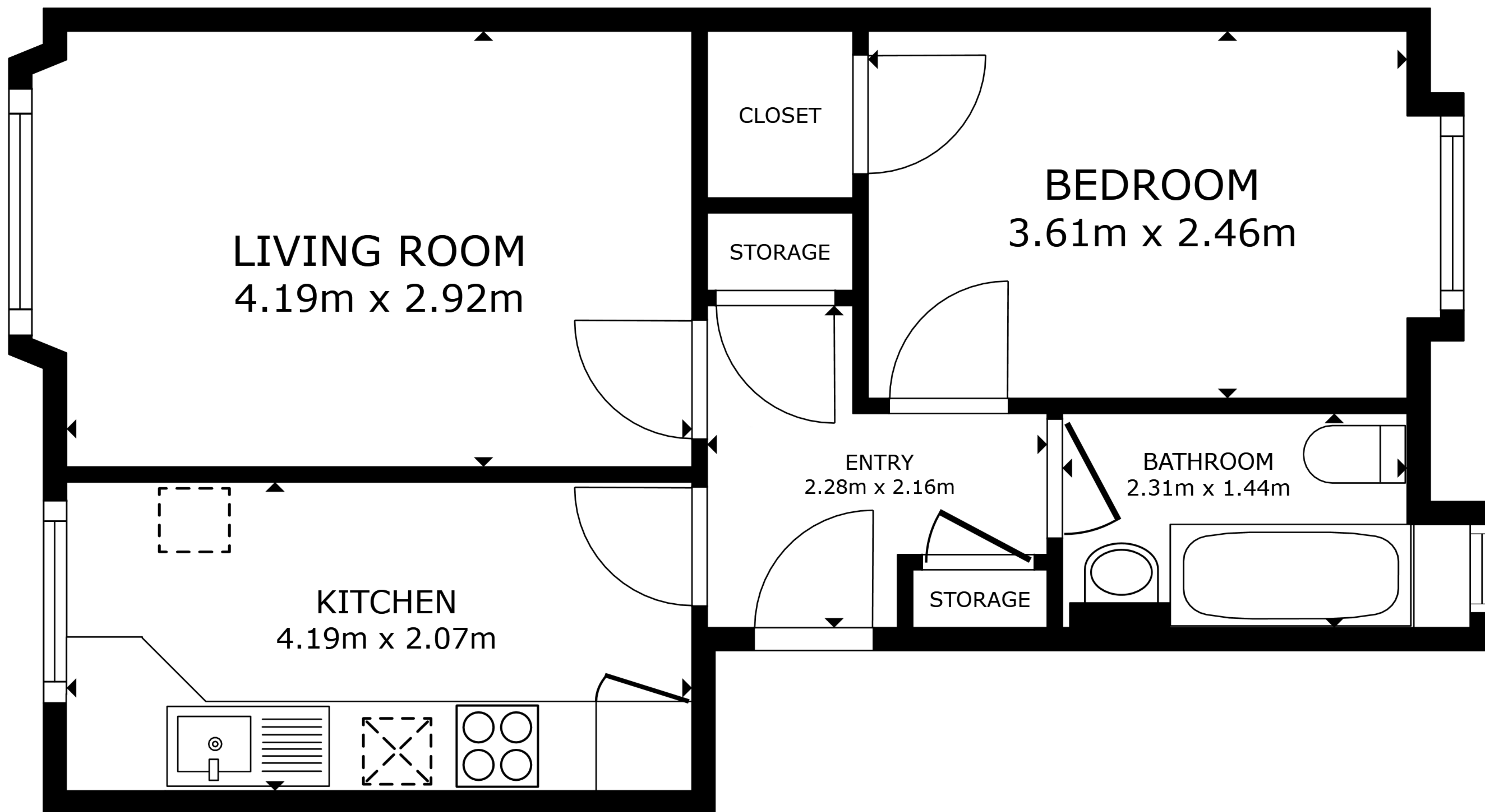
FLOOR PLAN
