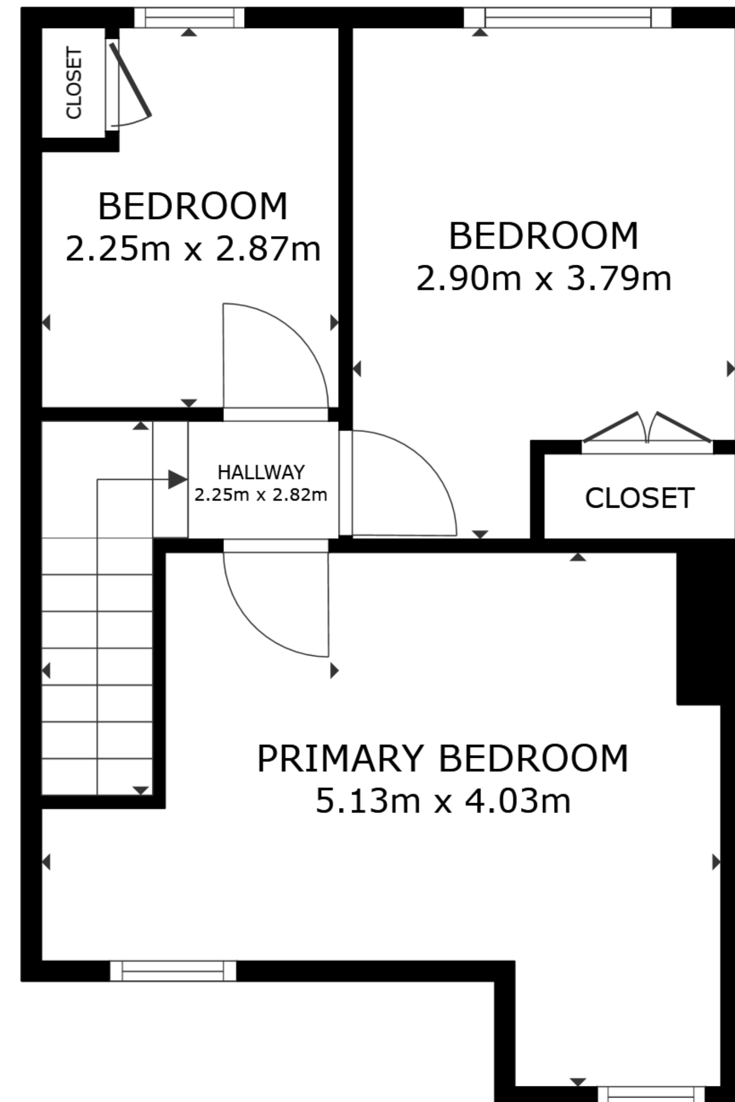
FLOOR 2
