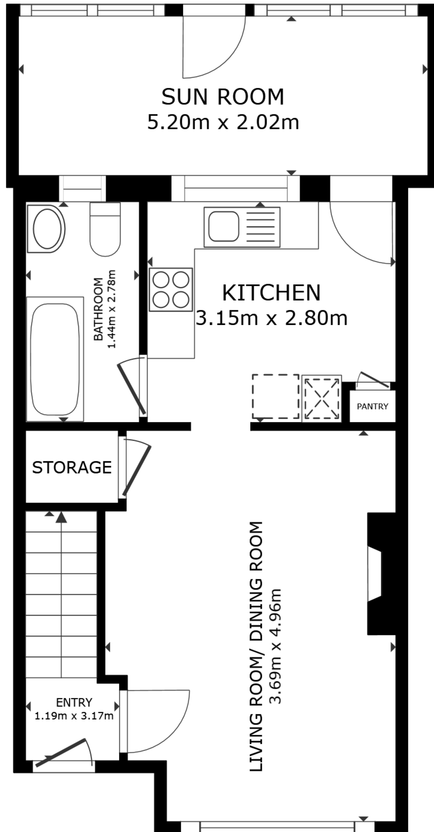
FLOOR 1
