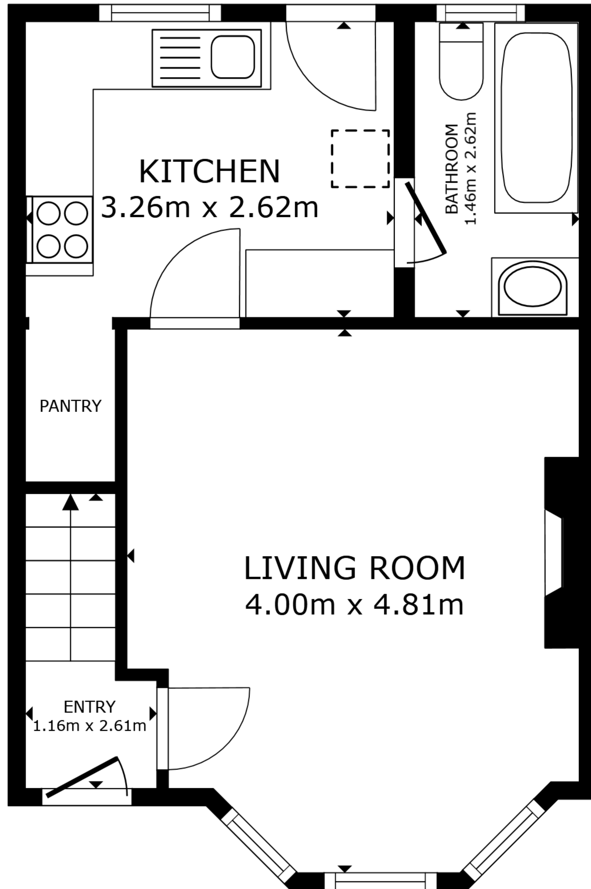
FLOOR 1
