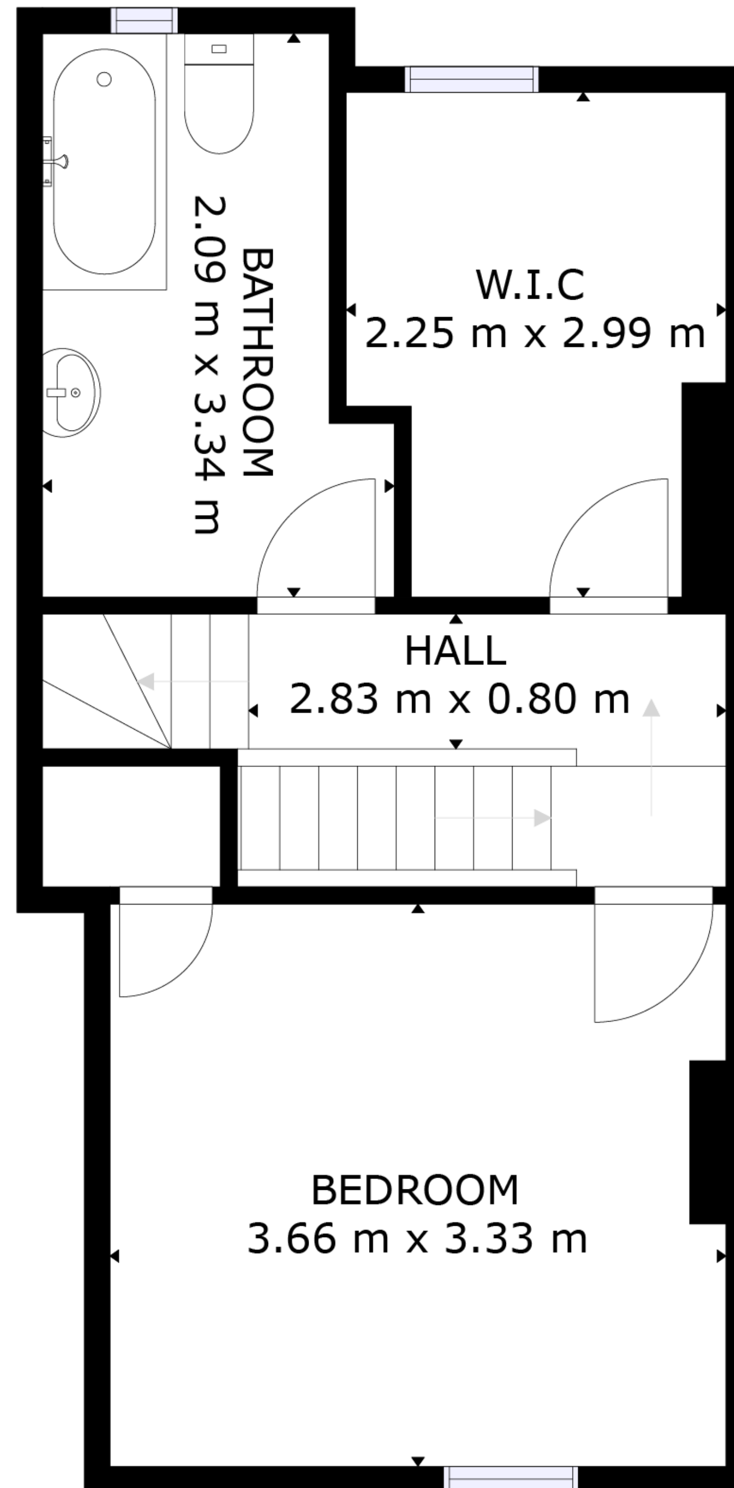
FLOOR 2
