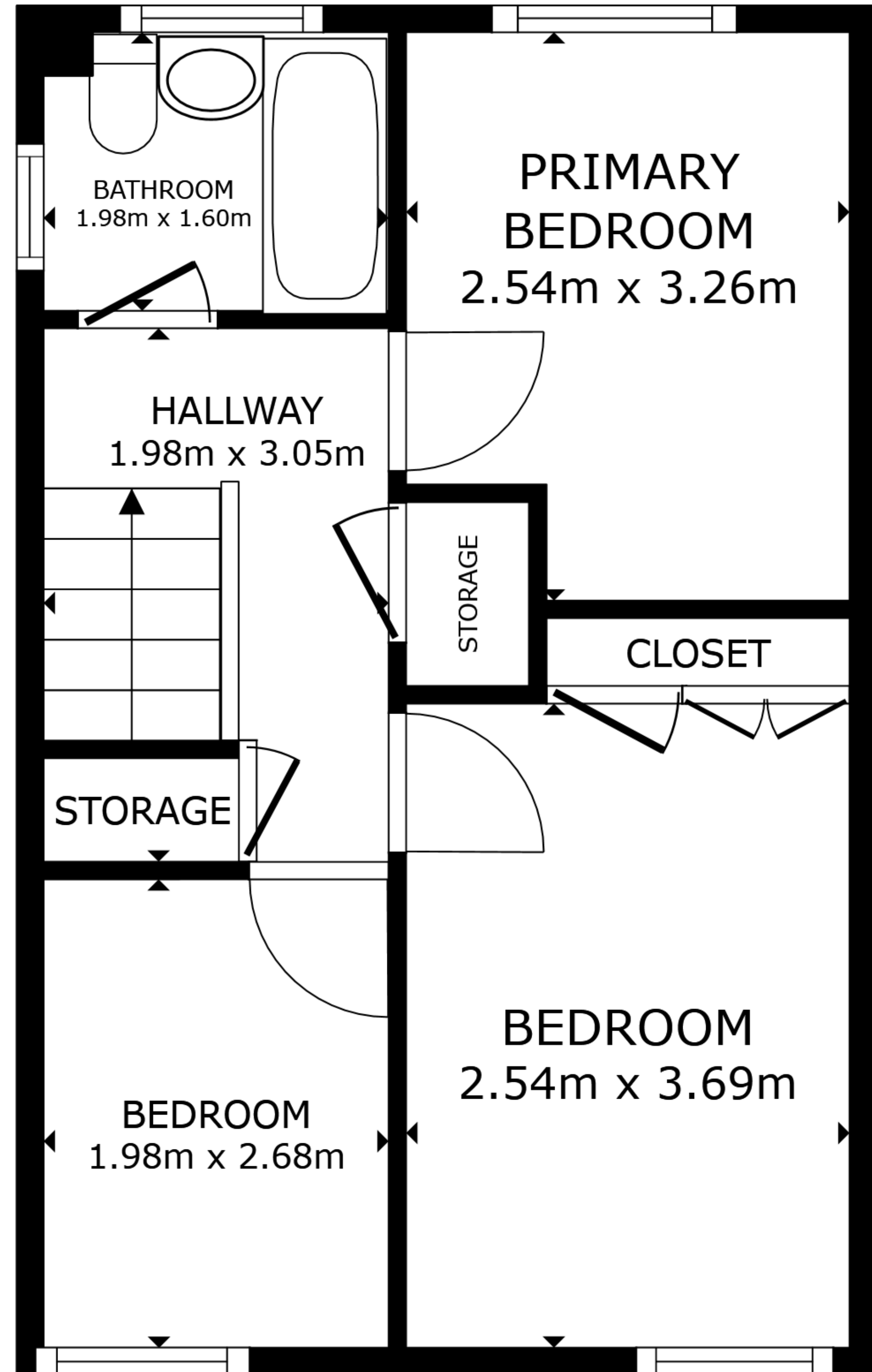
FLOOR 2
