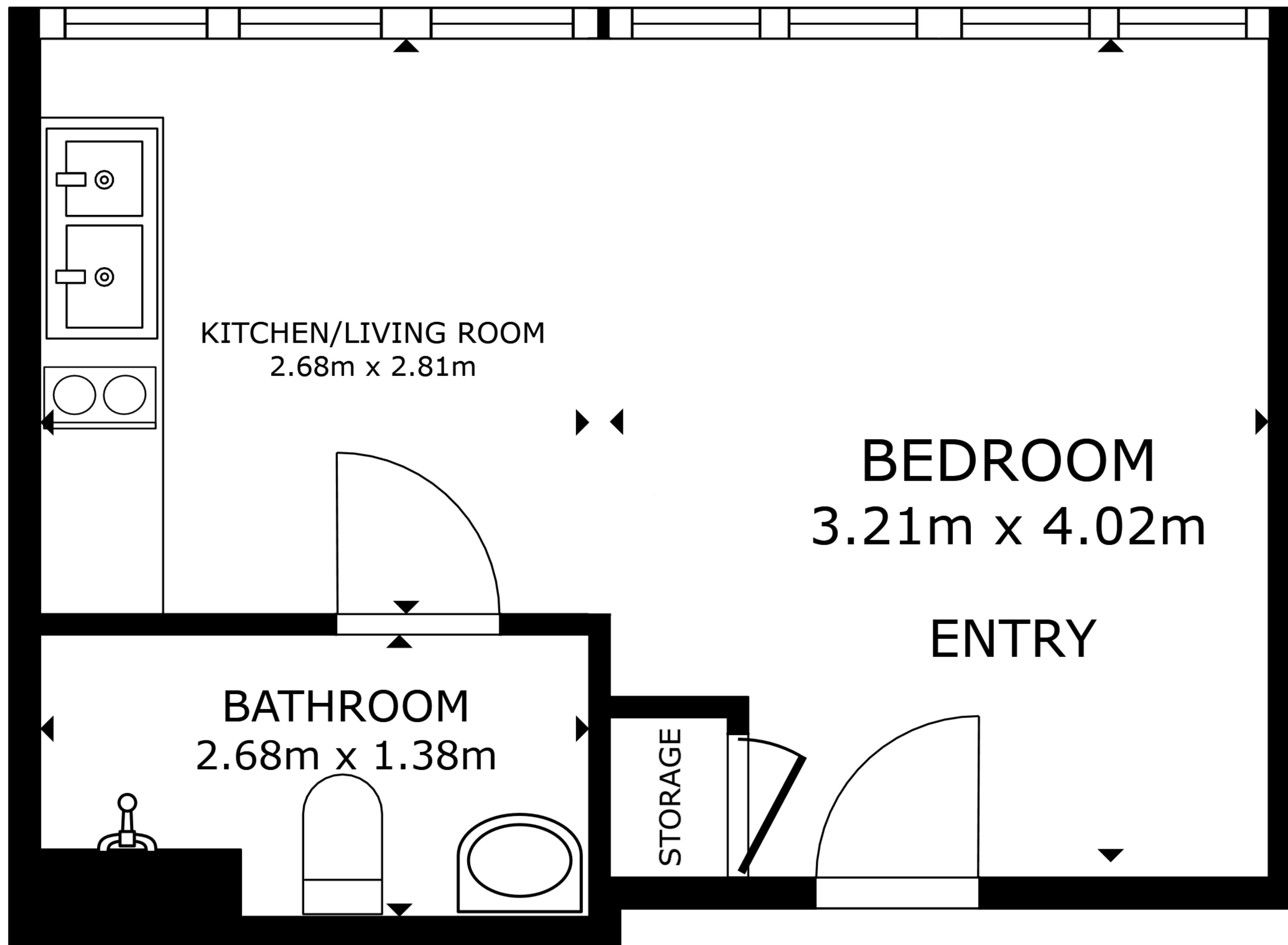
FLOOR PLAN
