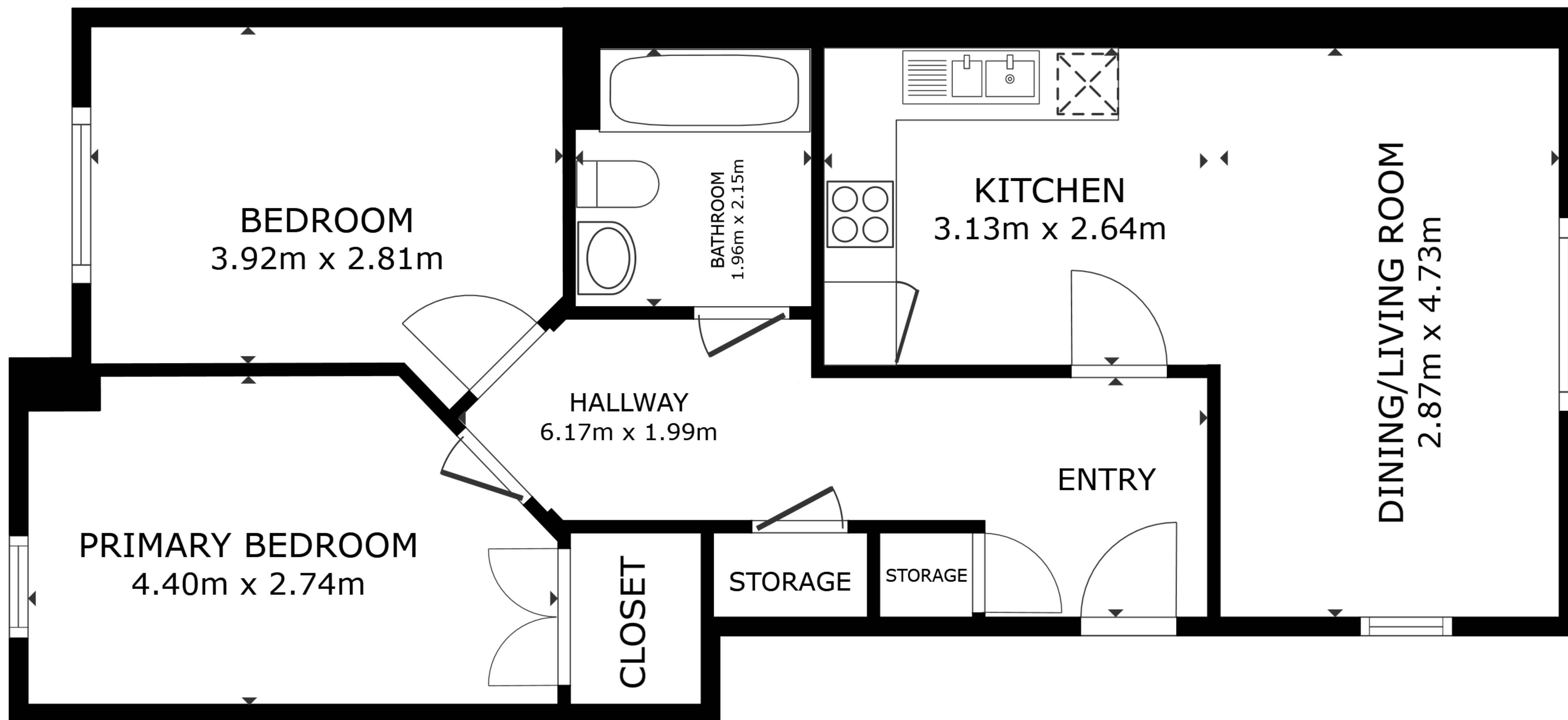
FLOOR PLAN
