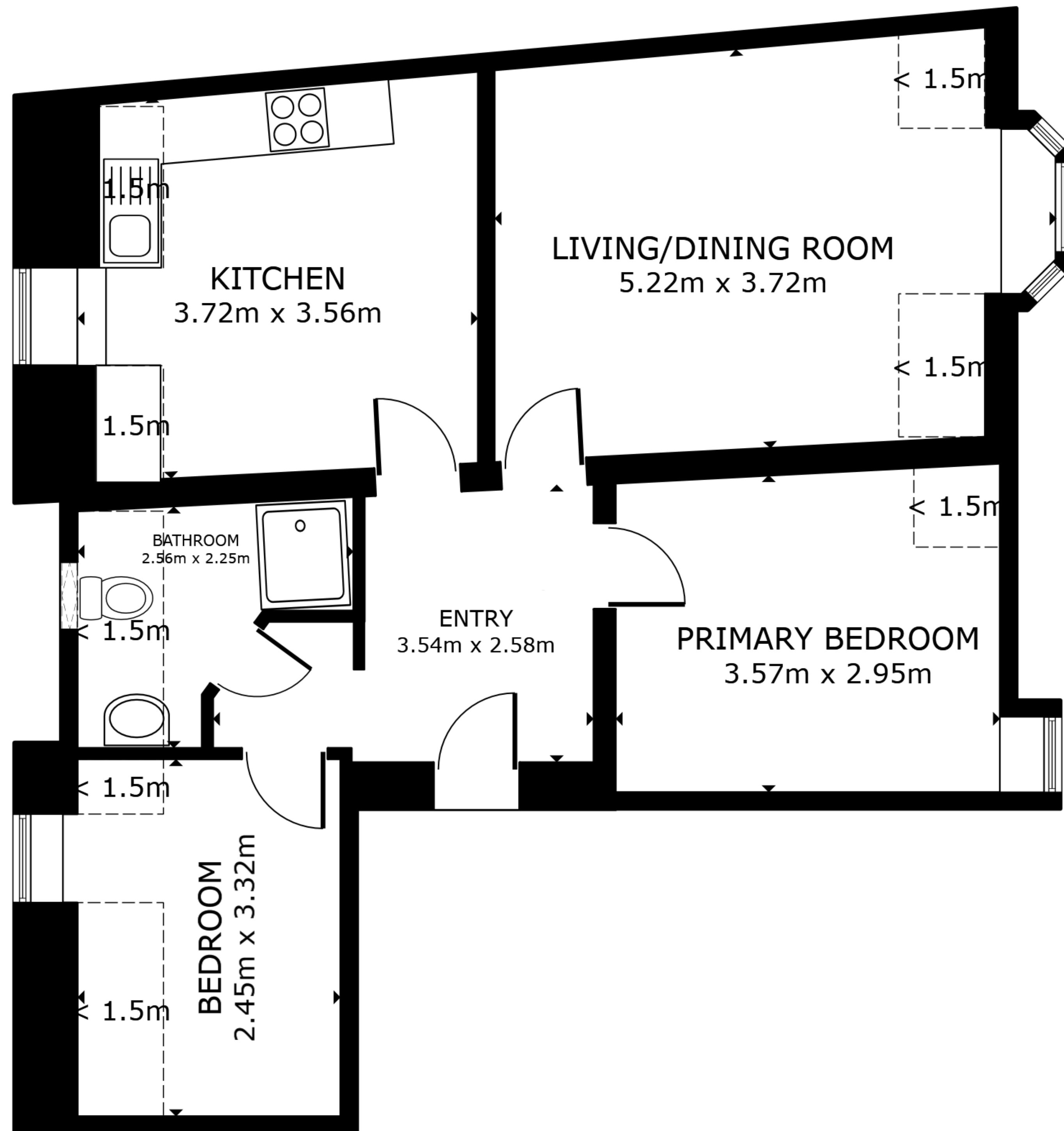
FLOOR PLAN
