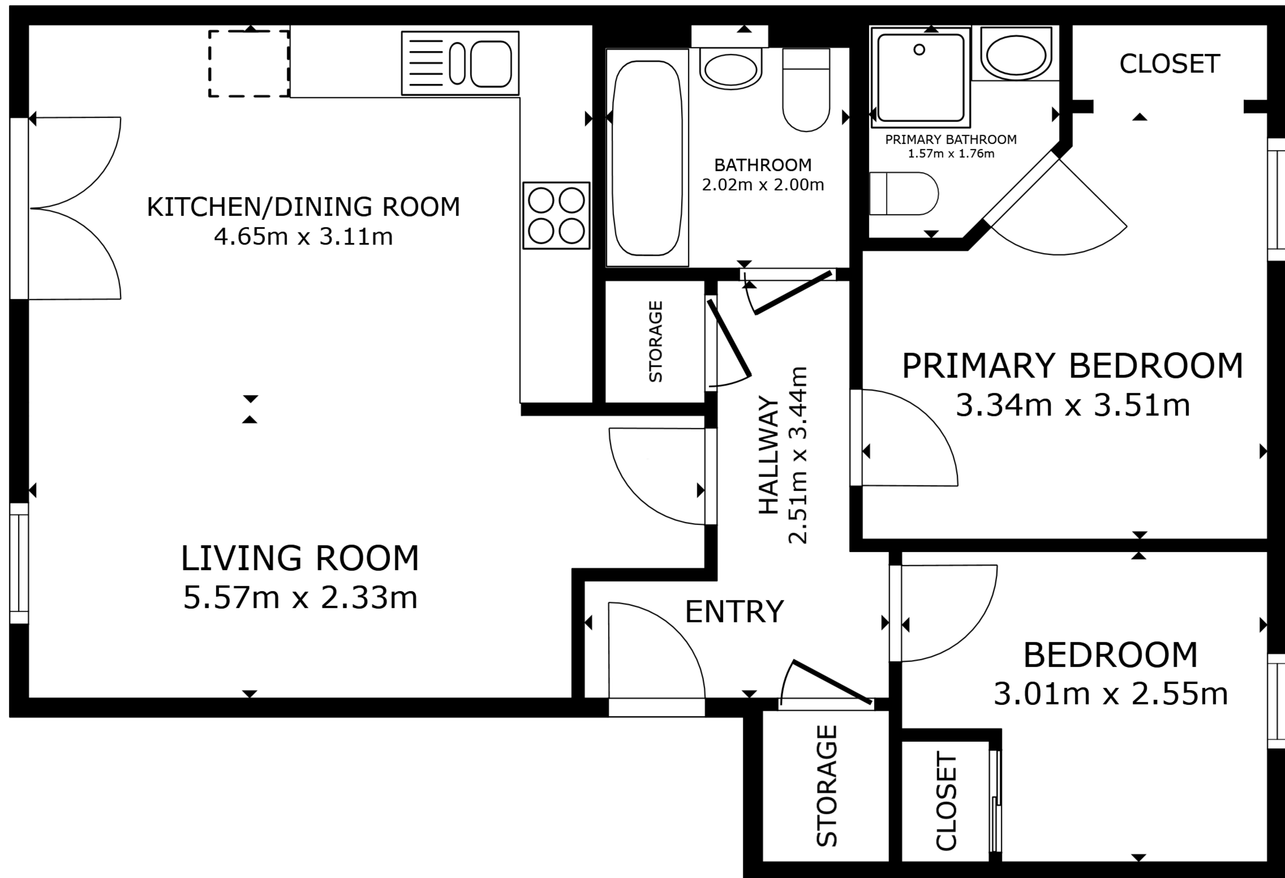
FLOOR PLAN
