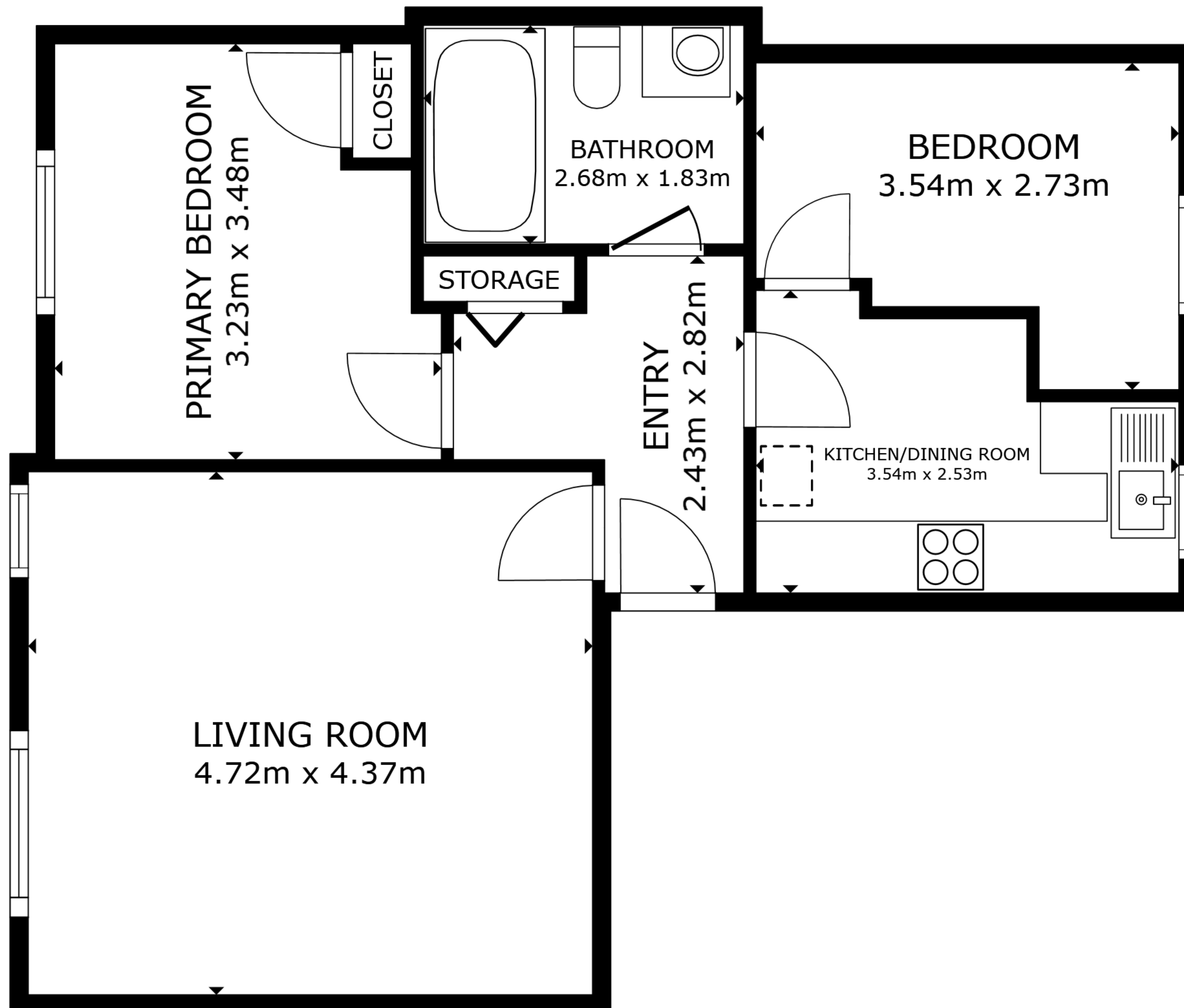
FLOOR PLAN
