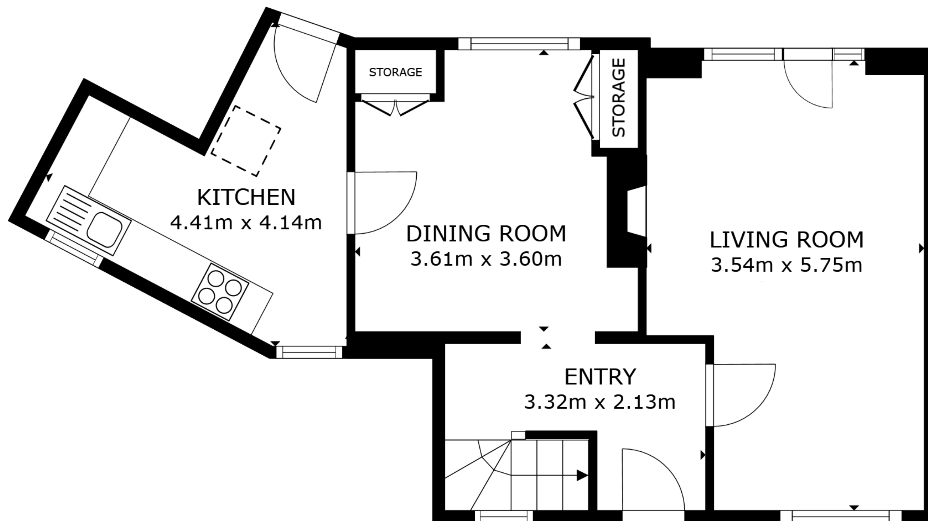
FLOOR 1
