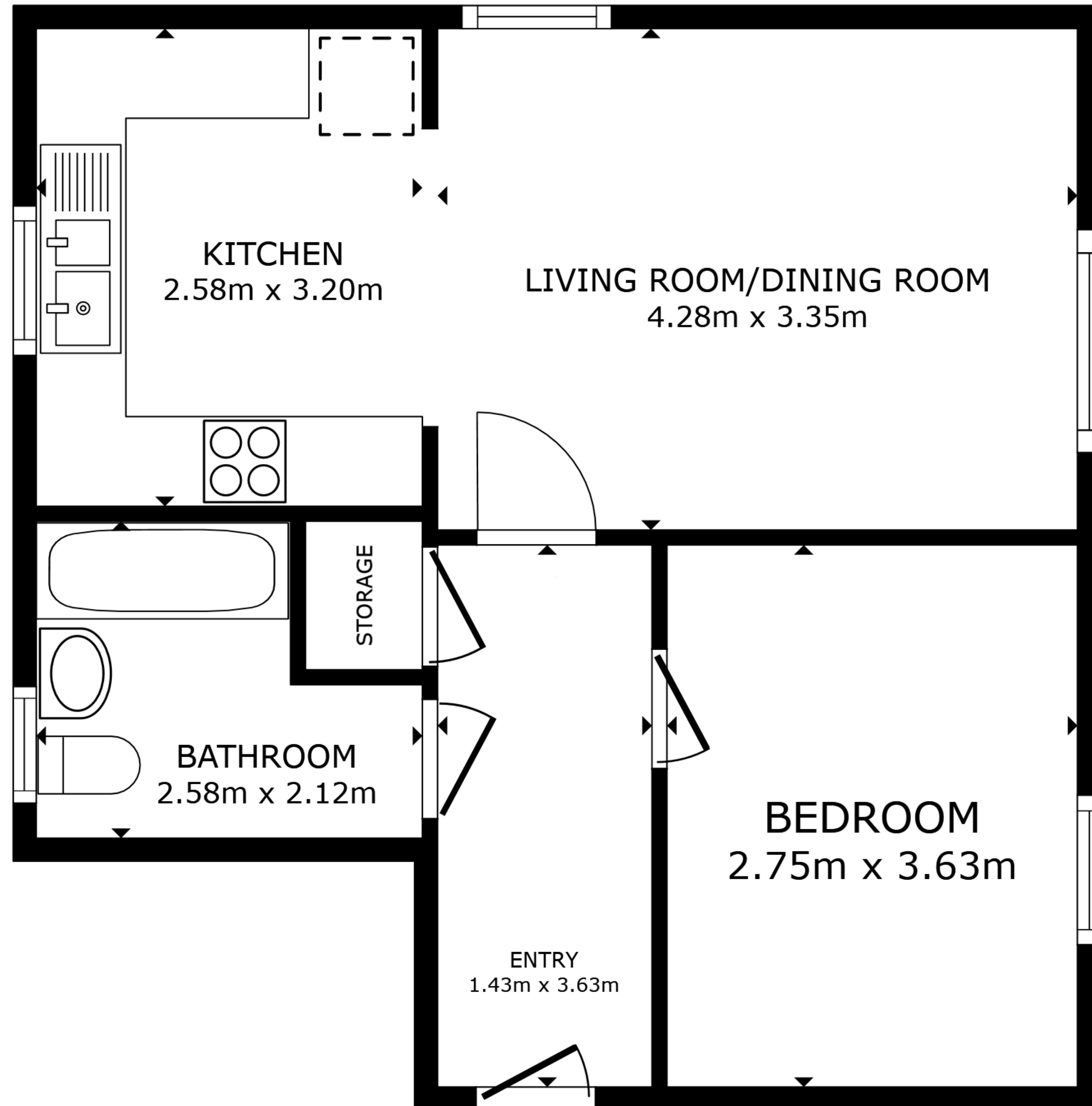
FLOOR PLAN
