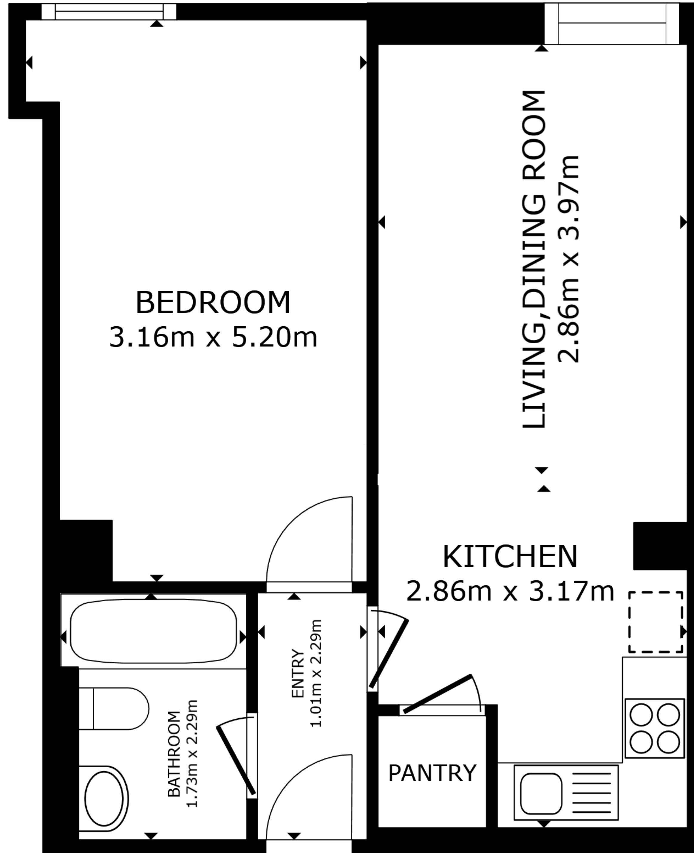
FLOOR PLAN
