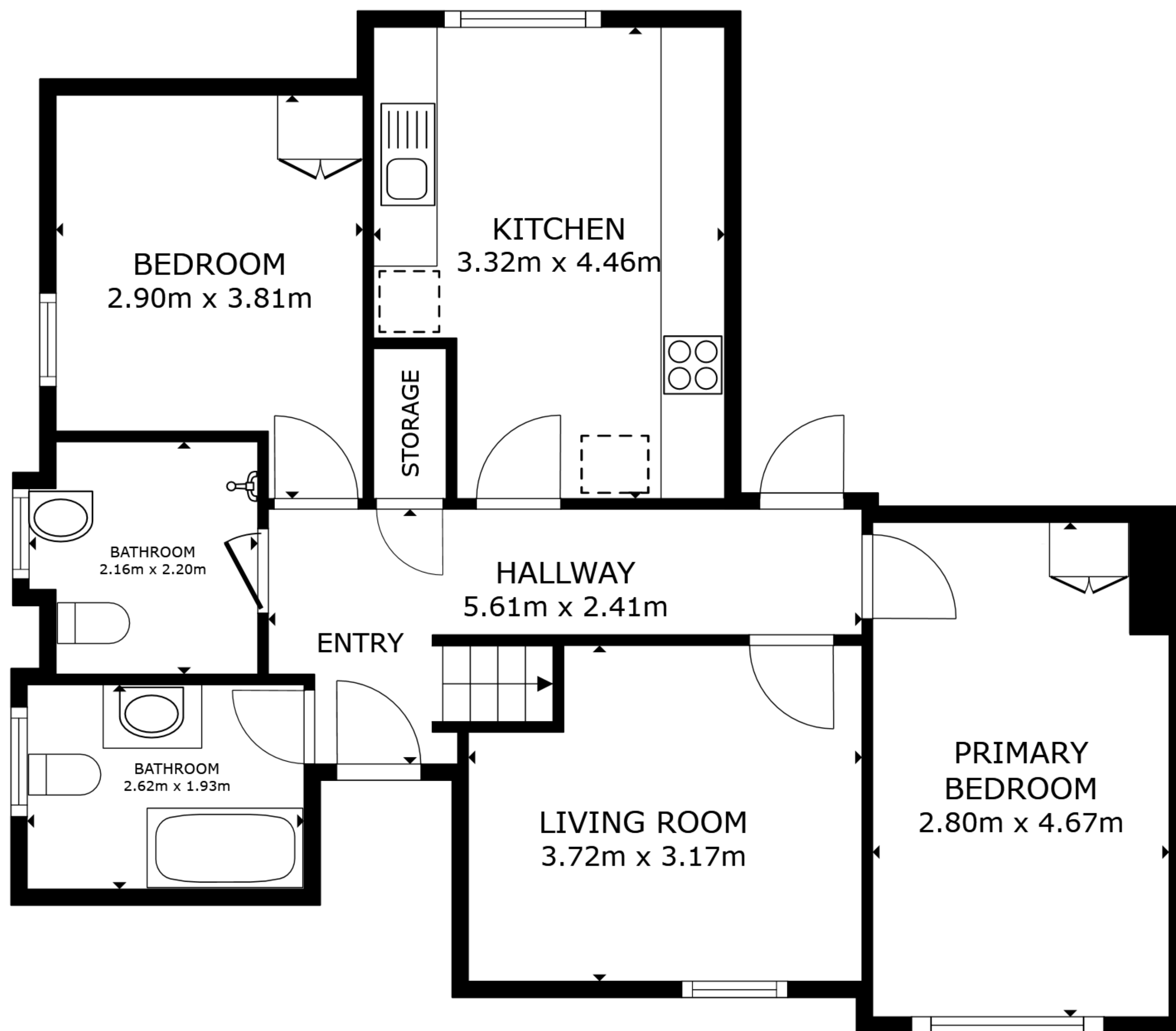
FLOOR 1
