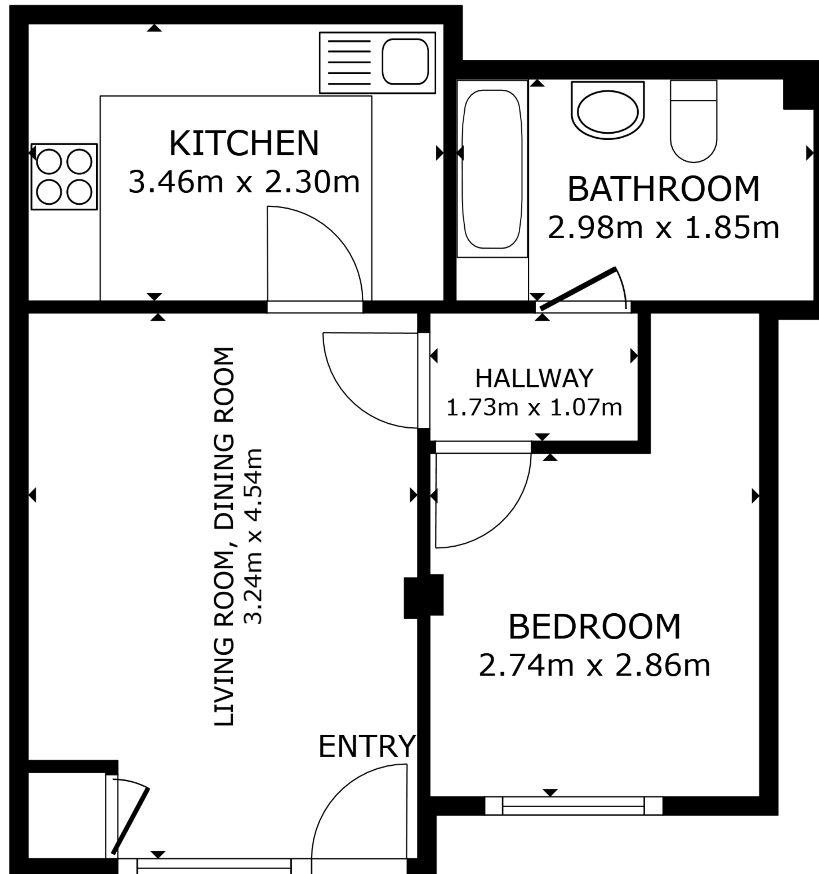
FLOOR PLAN
