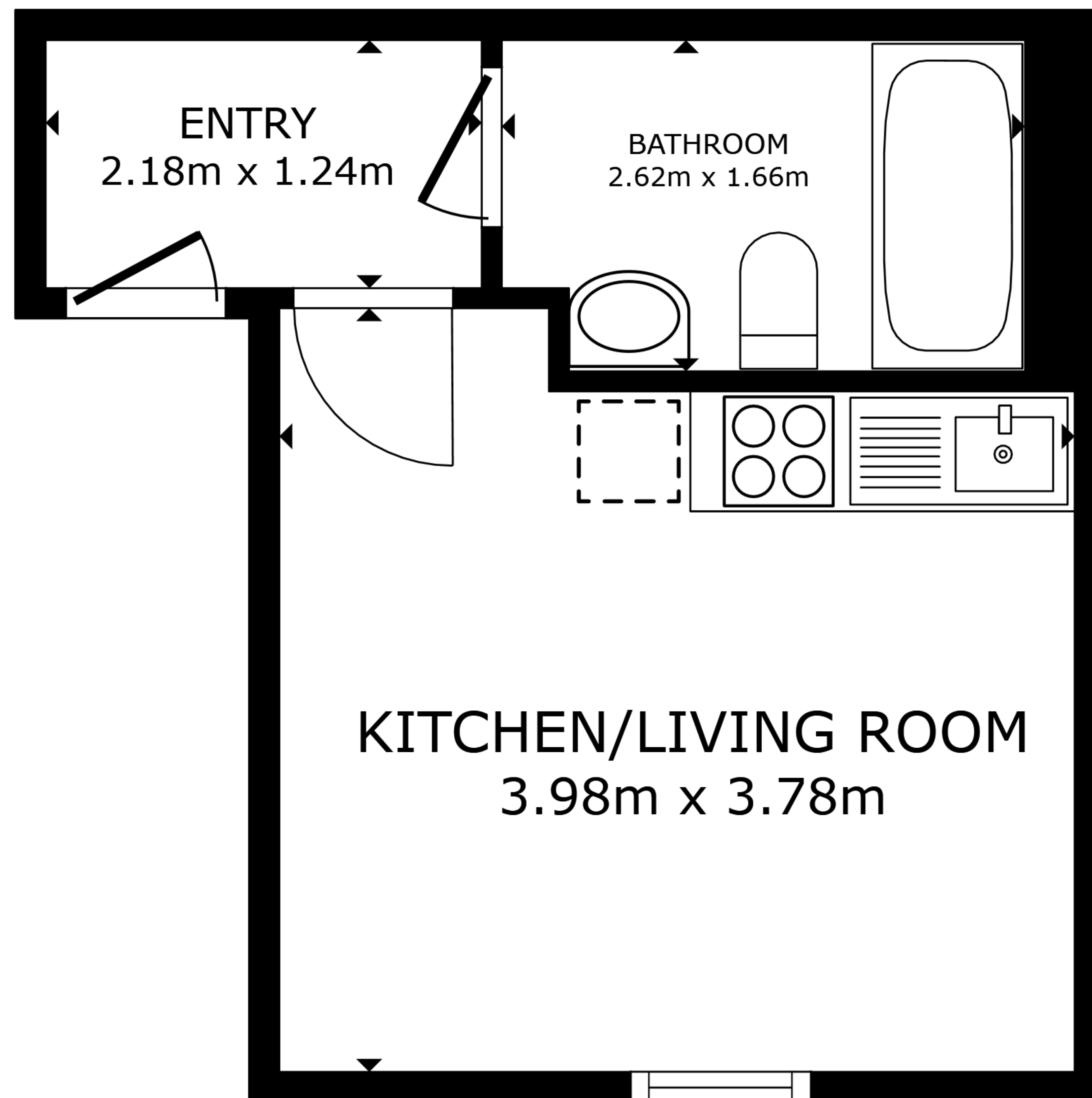
FLOOR PLAN
