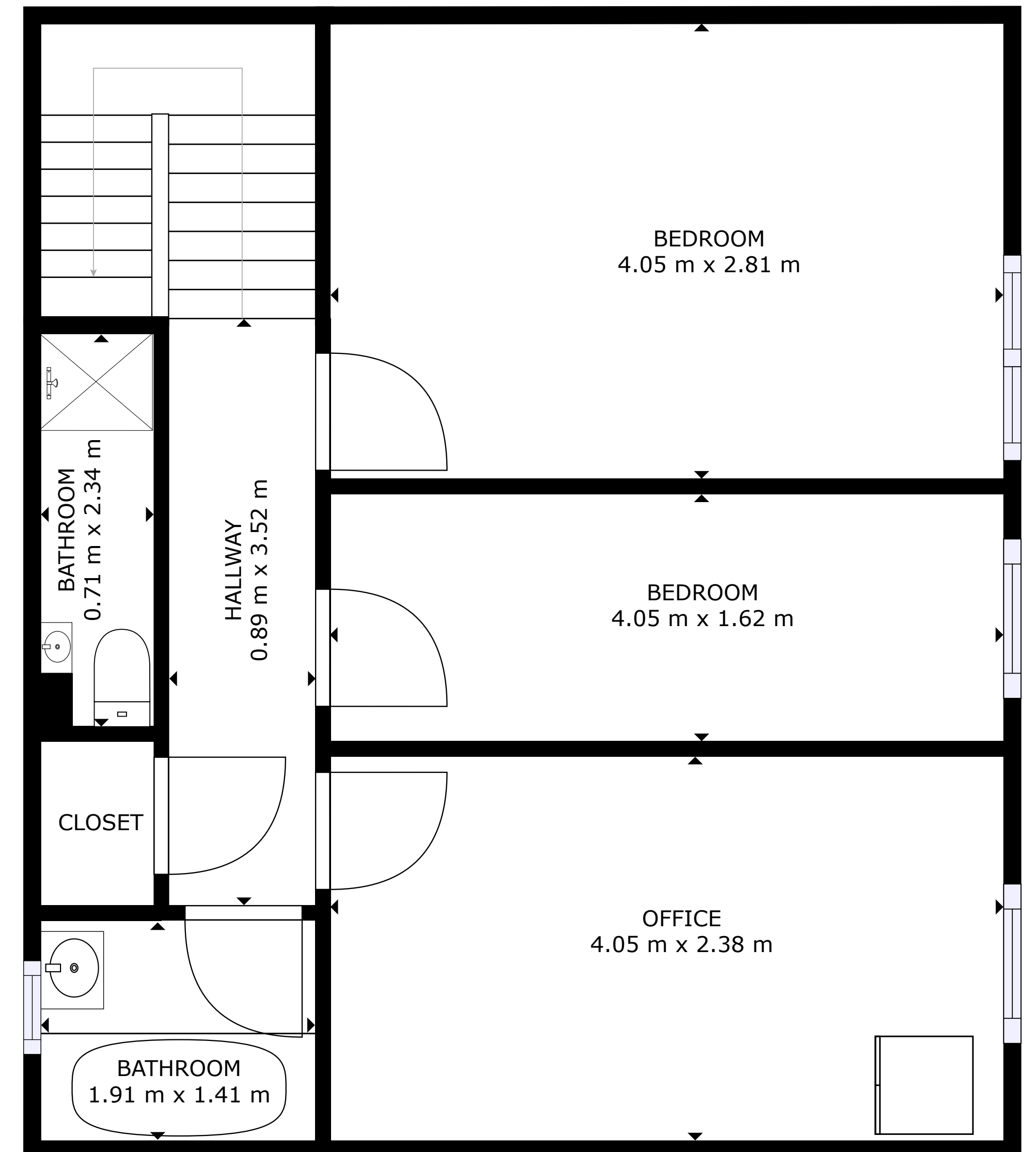
FLOOR 2
