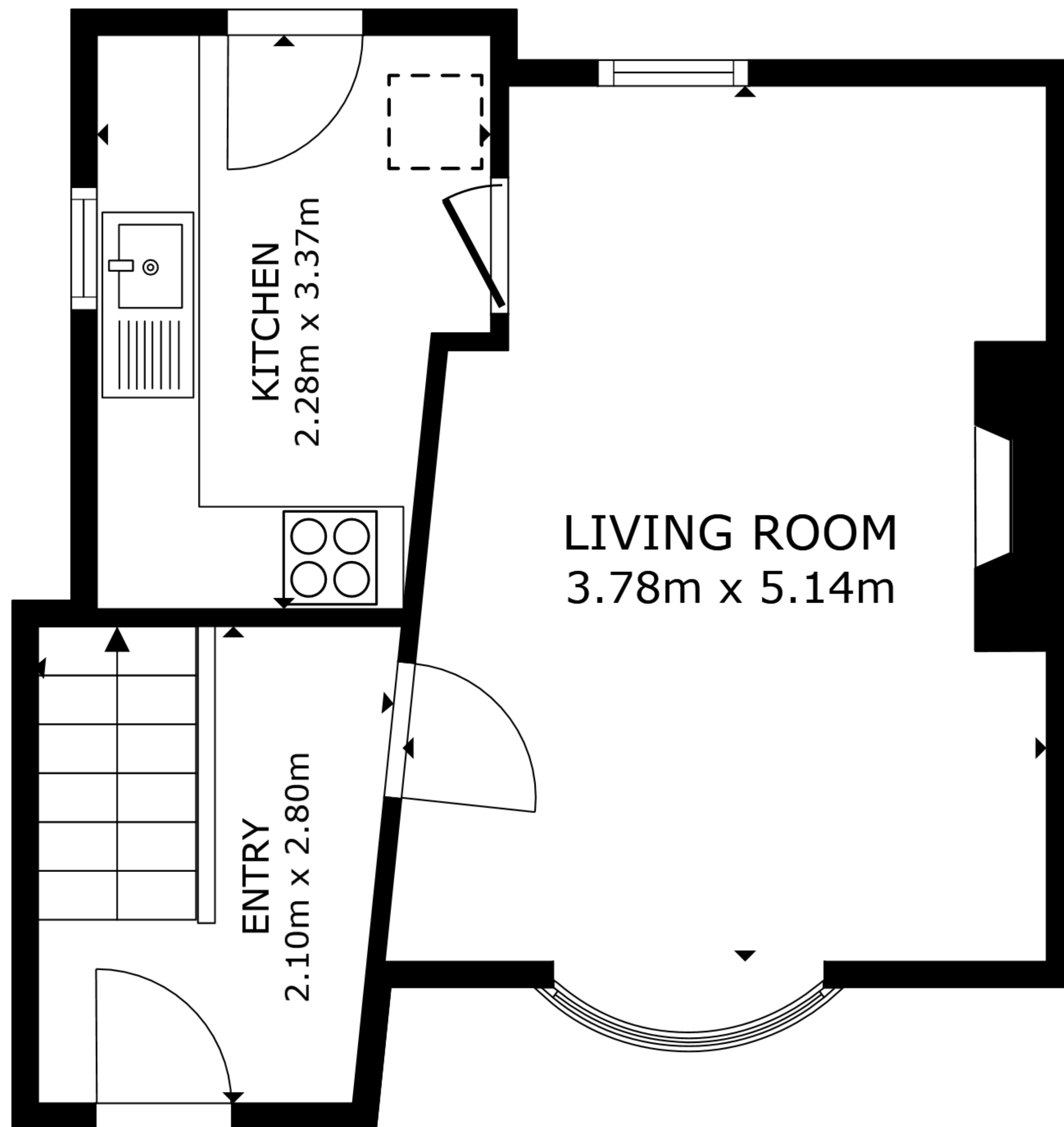
FLOOR 1
