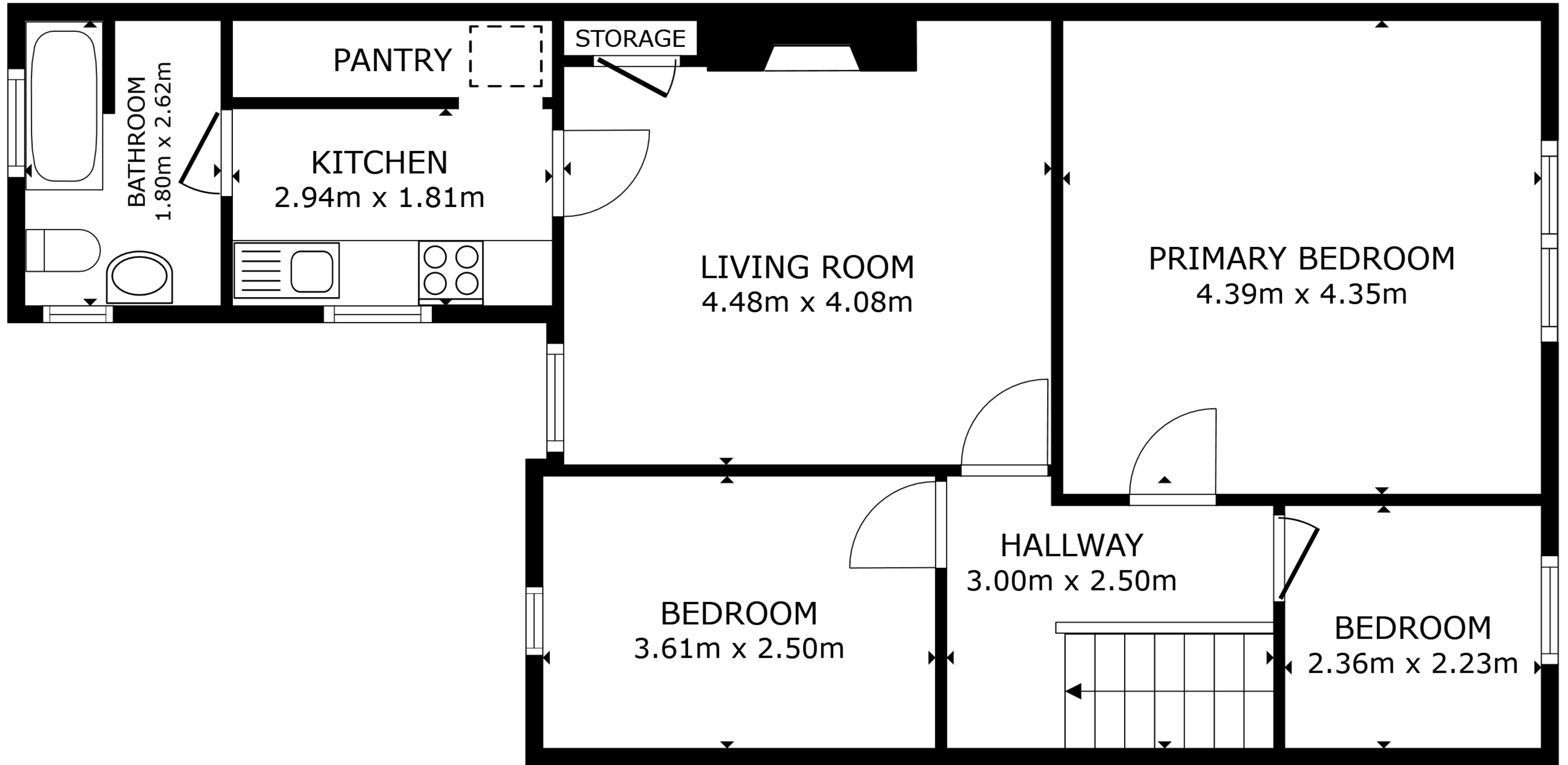
FLOOR PLAN
