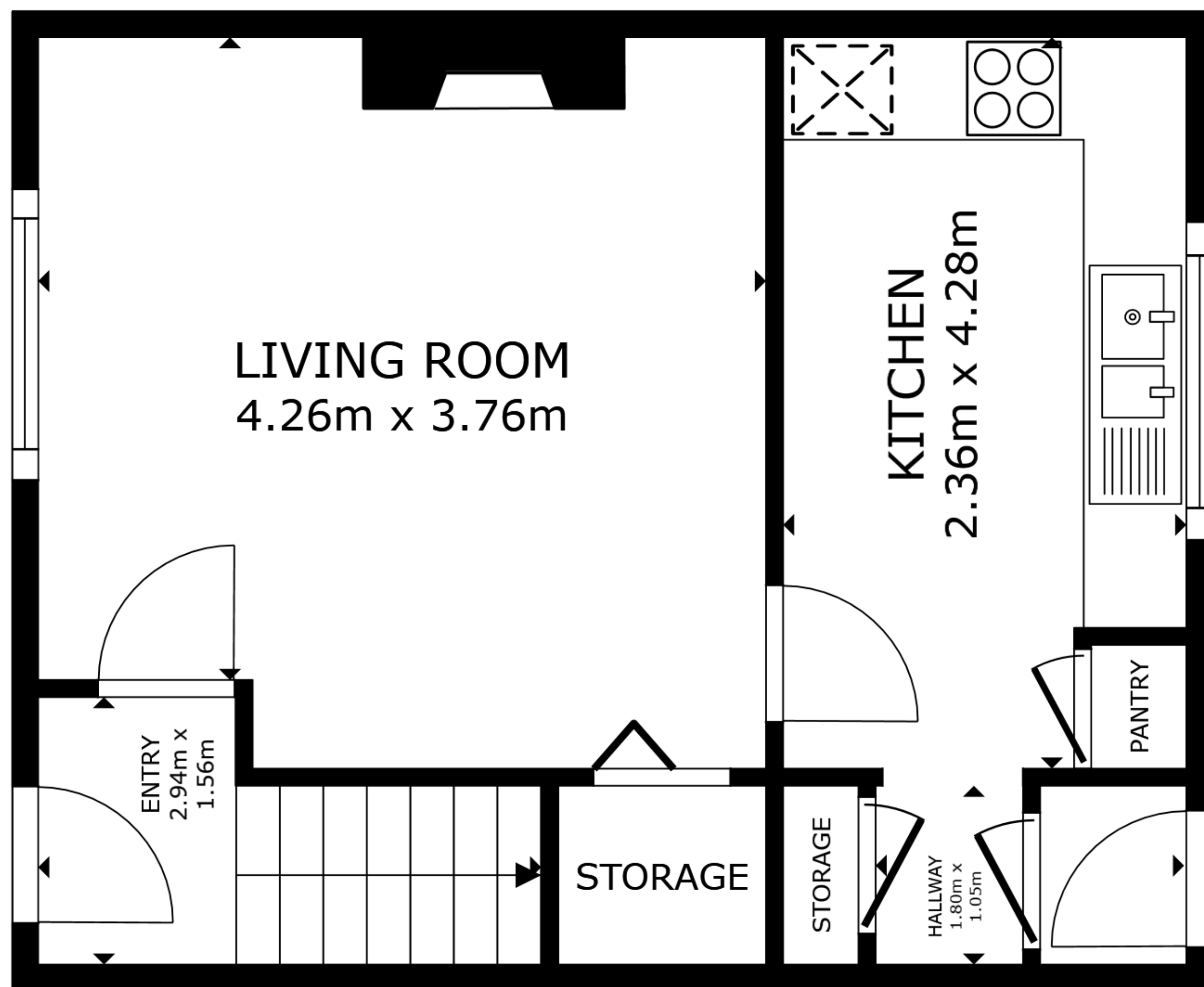
FLOOR 1
