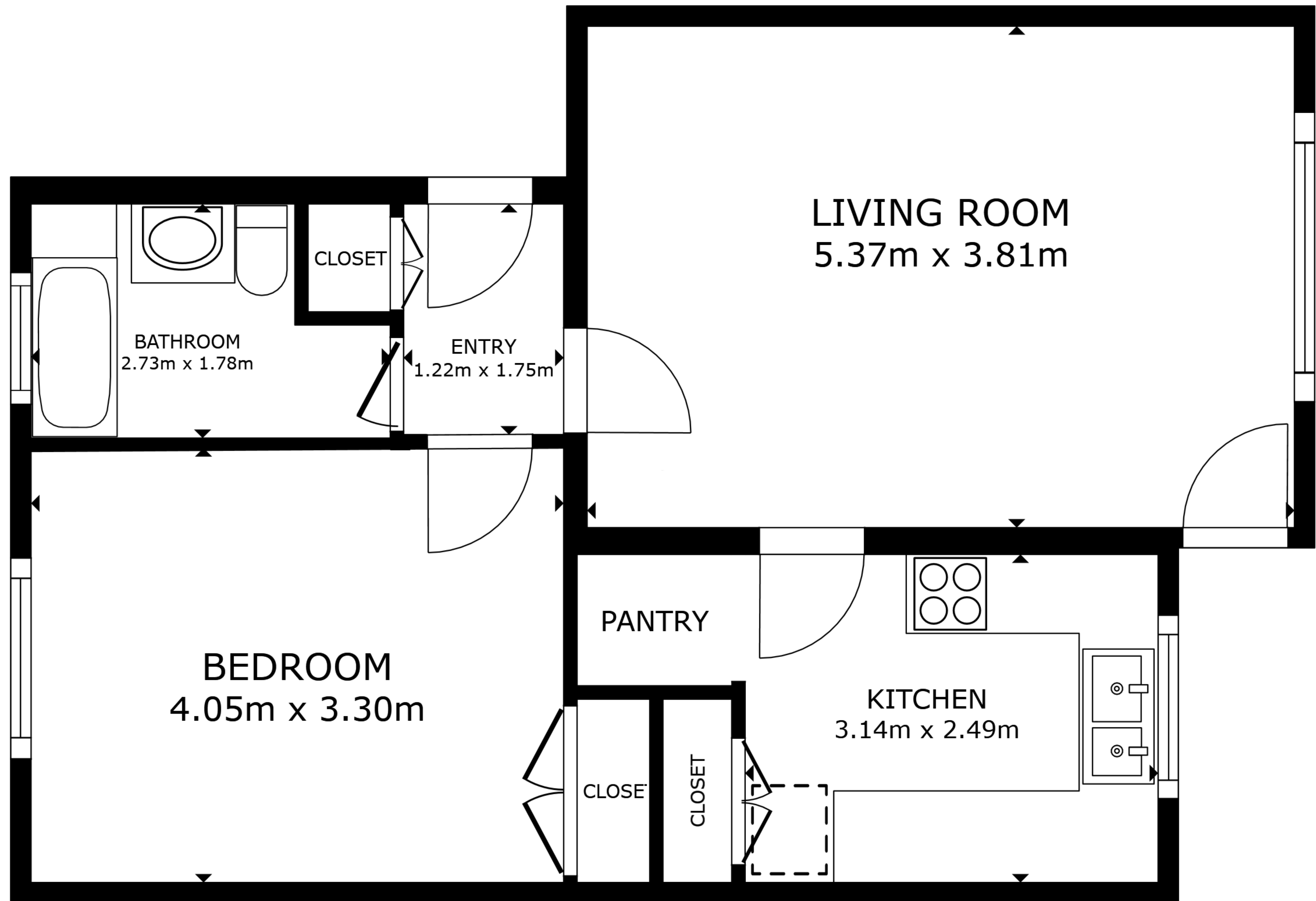
FLOOR PLAN
