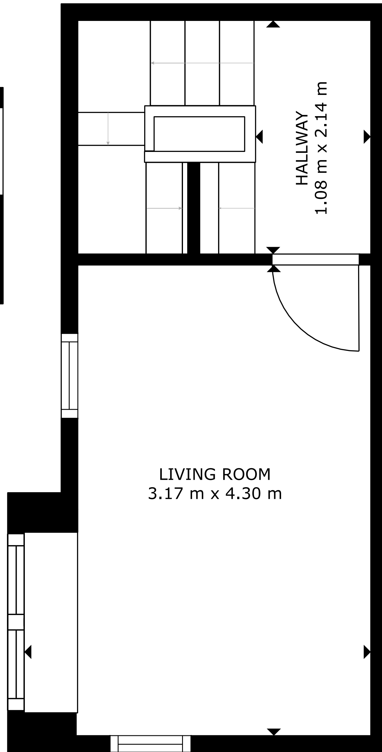
FLOOR 2
