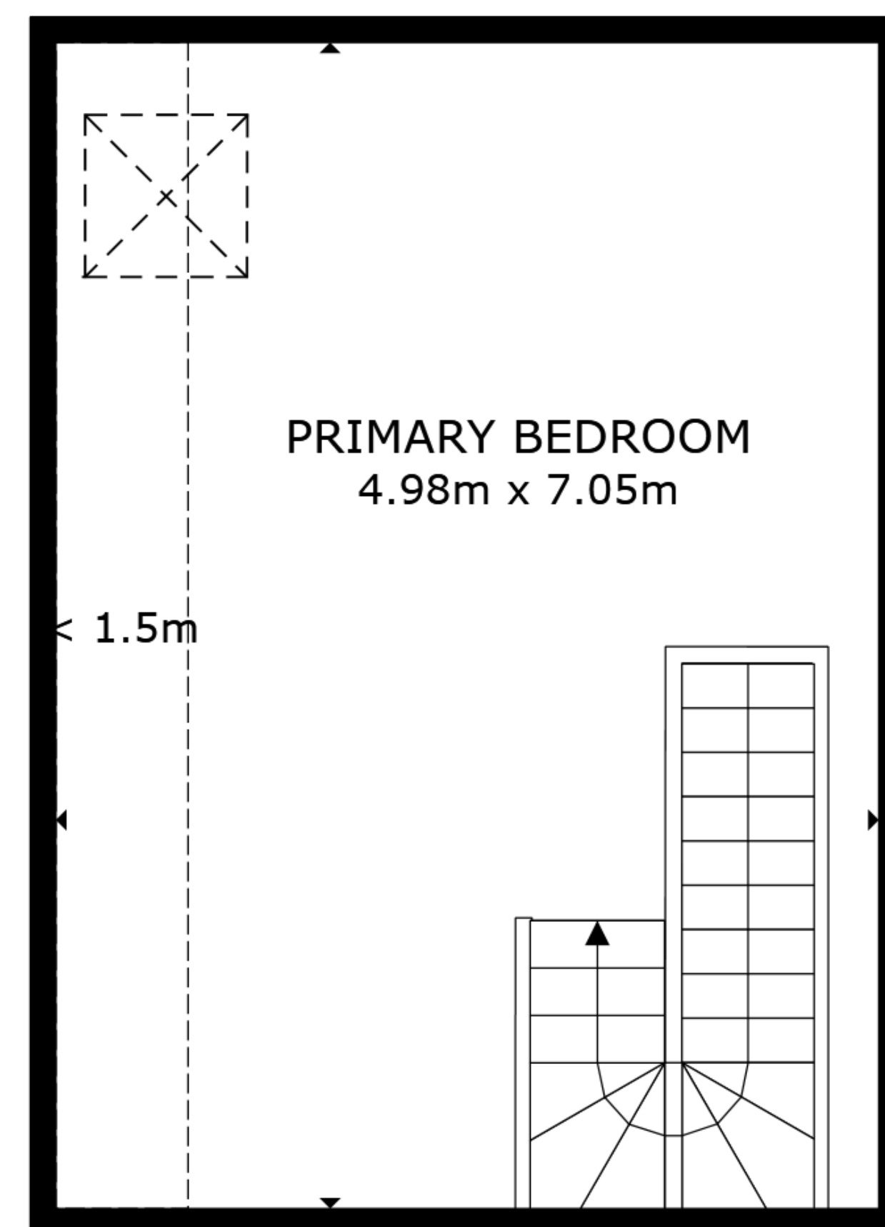
FLOOR 3
