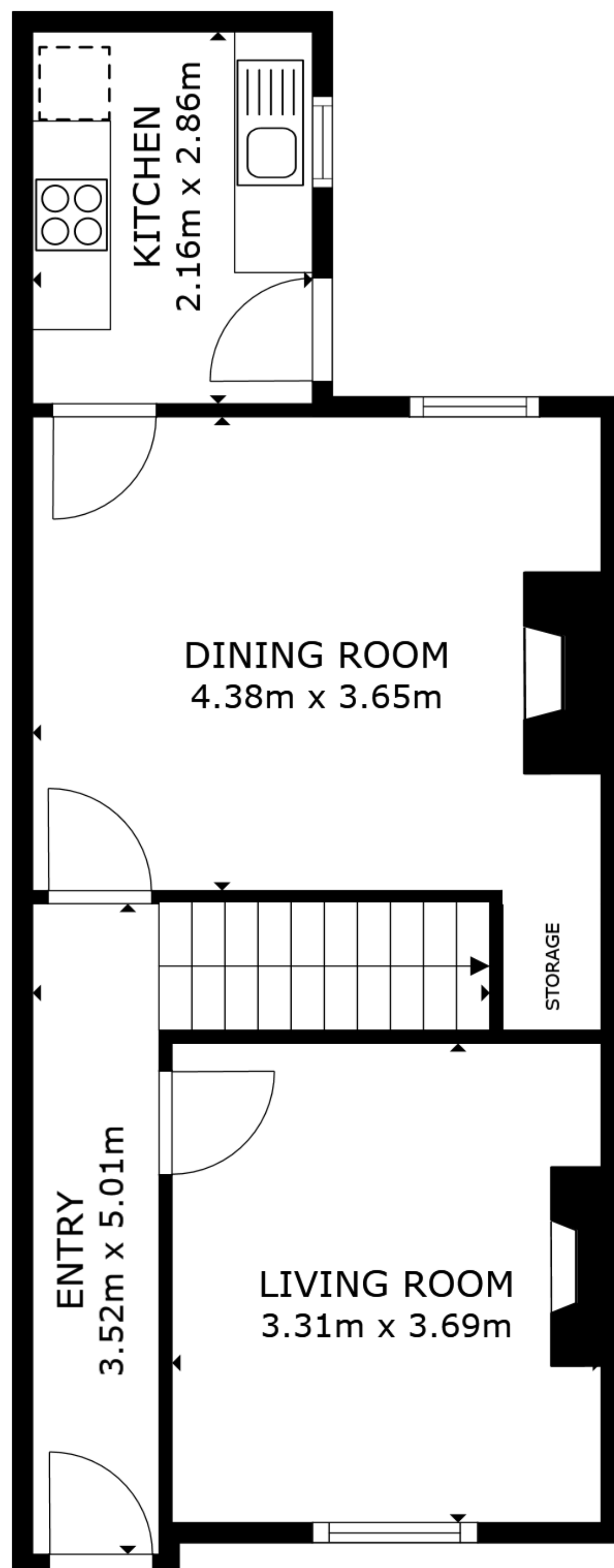
FLOOR 1
