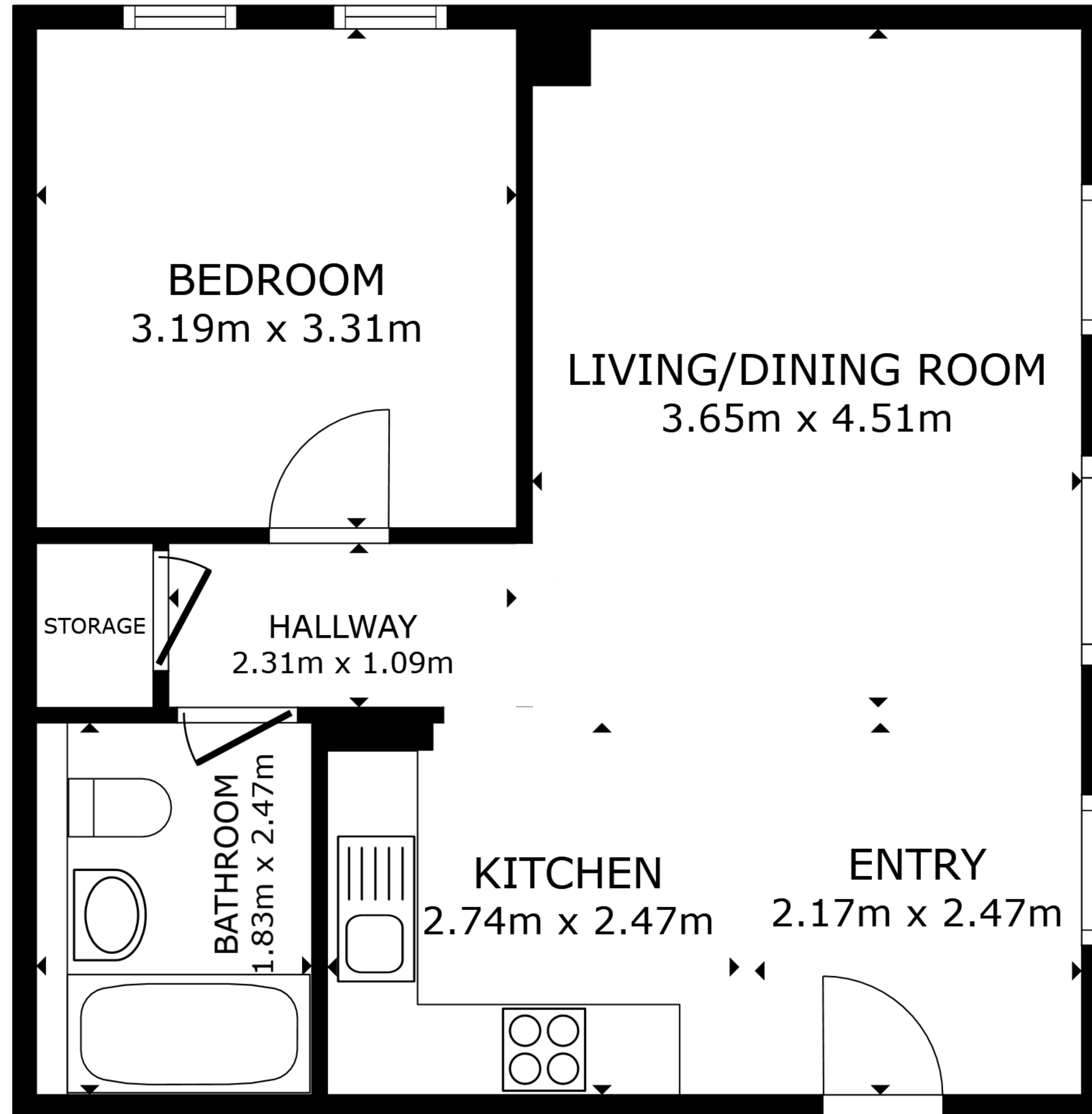
FLOOR PLAN
