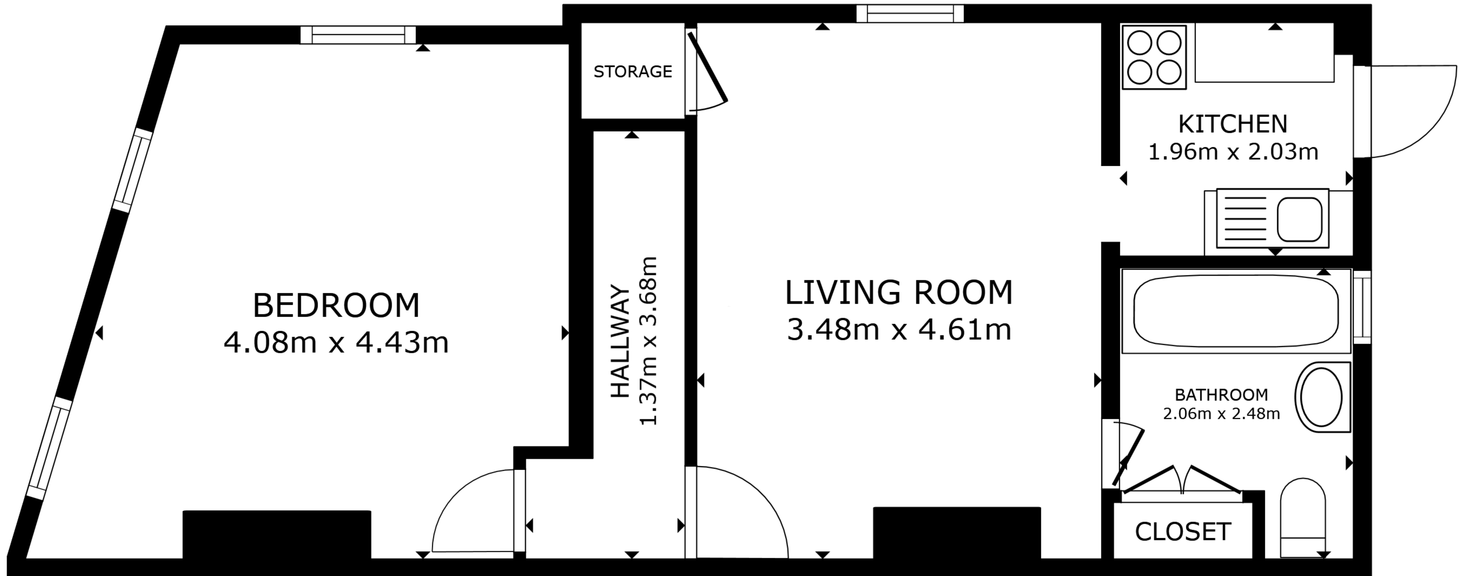
FLOOR PLAN
