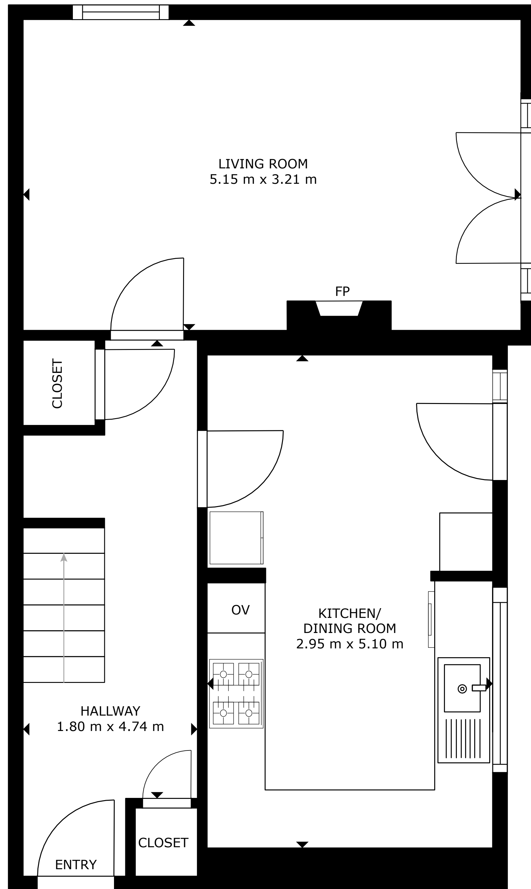
FLOOR 1
