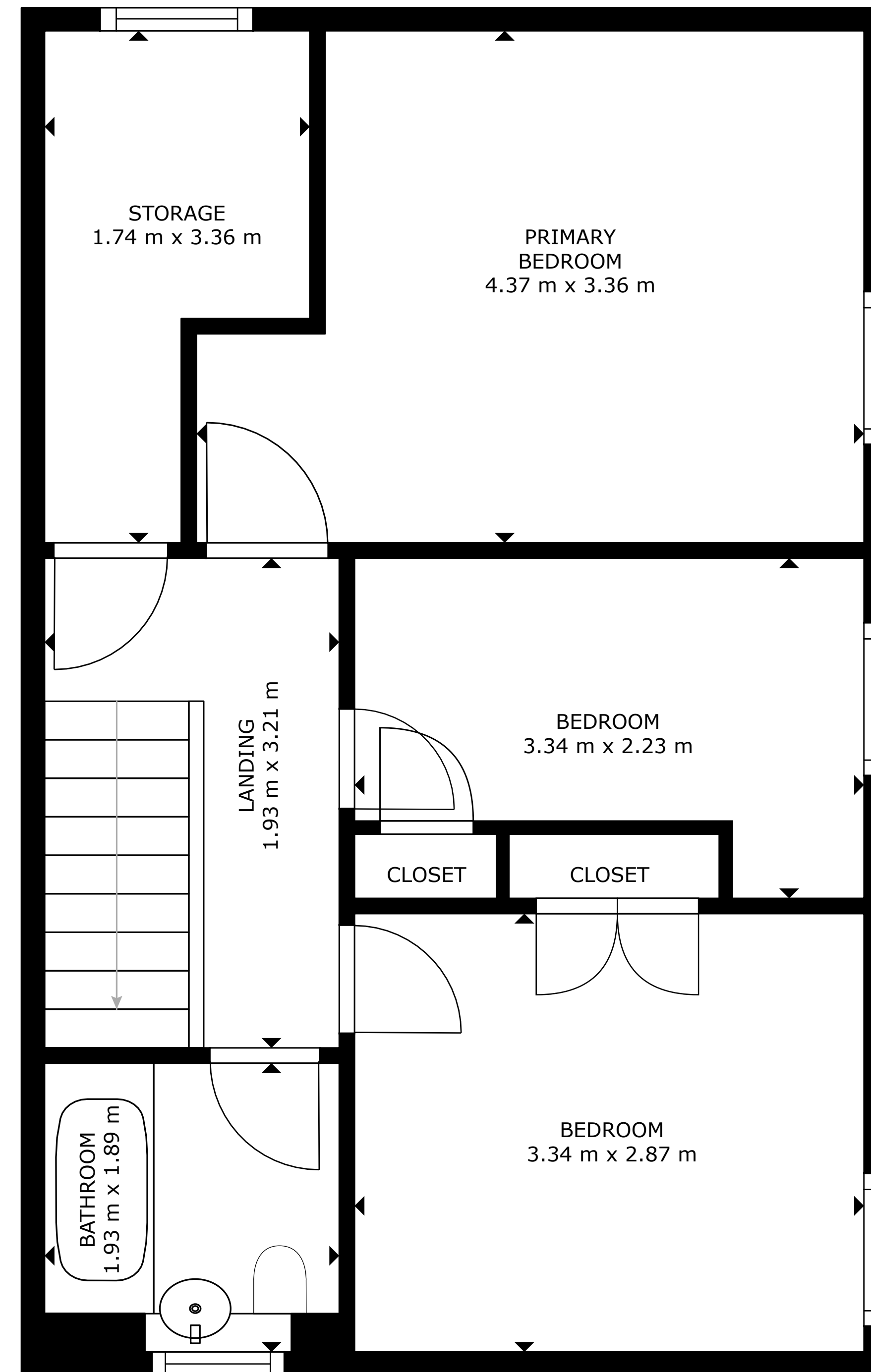
FLOOR 2
