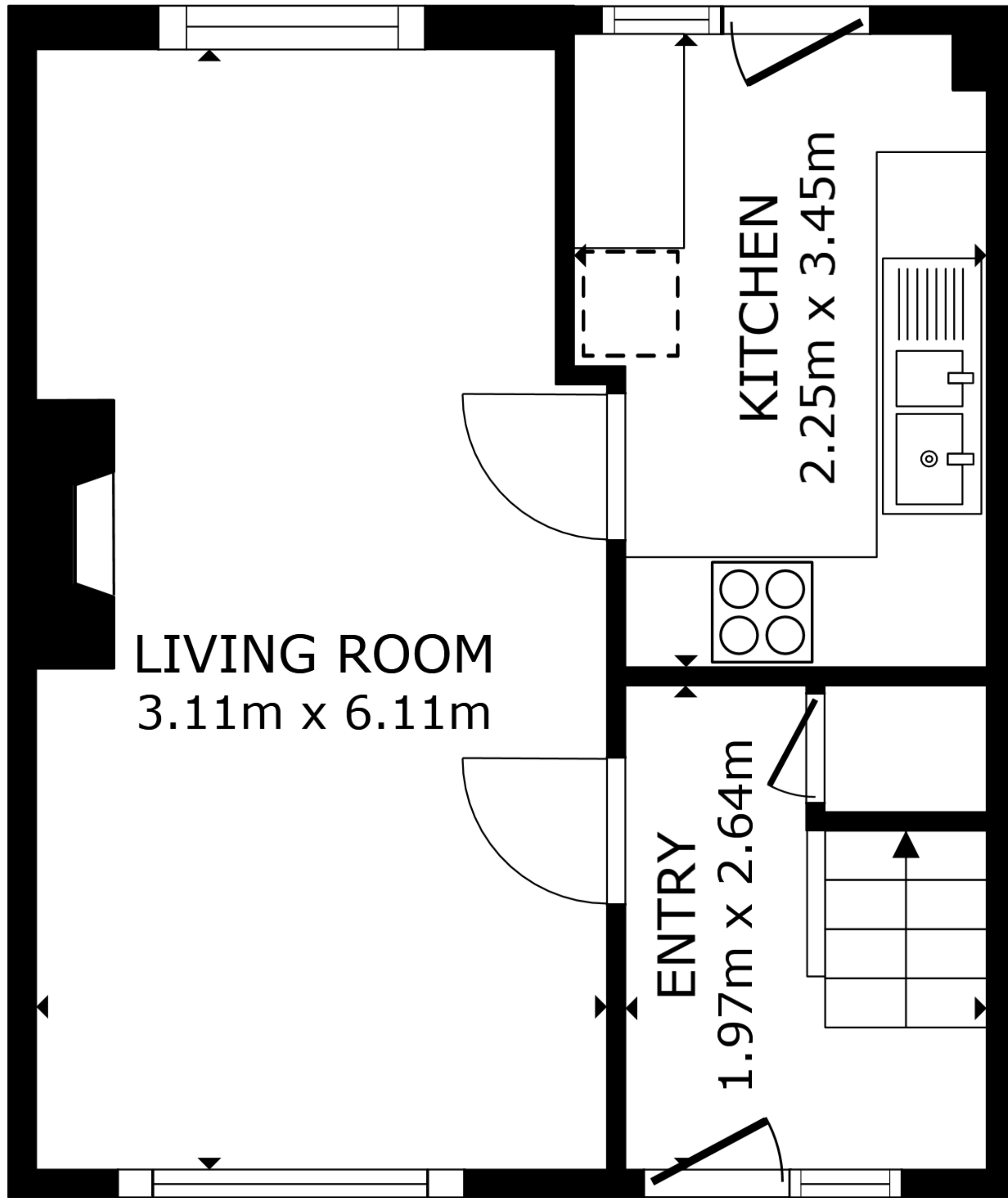
FLOOR 1
