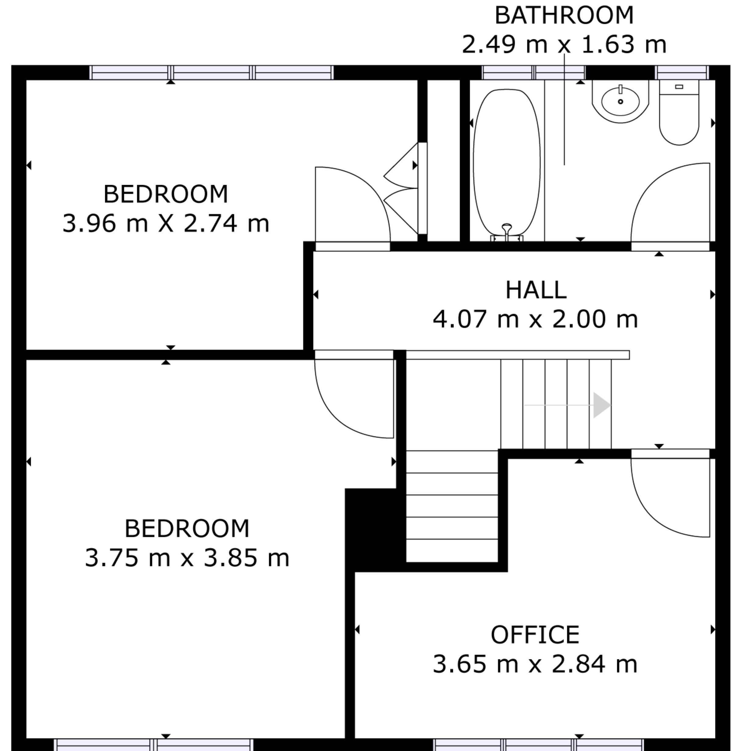
FLOOR 2
