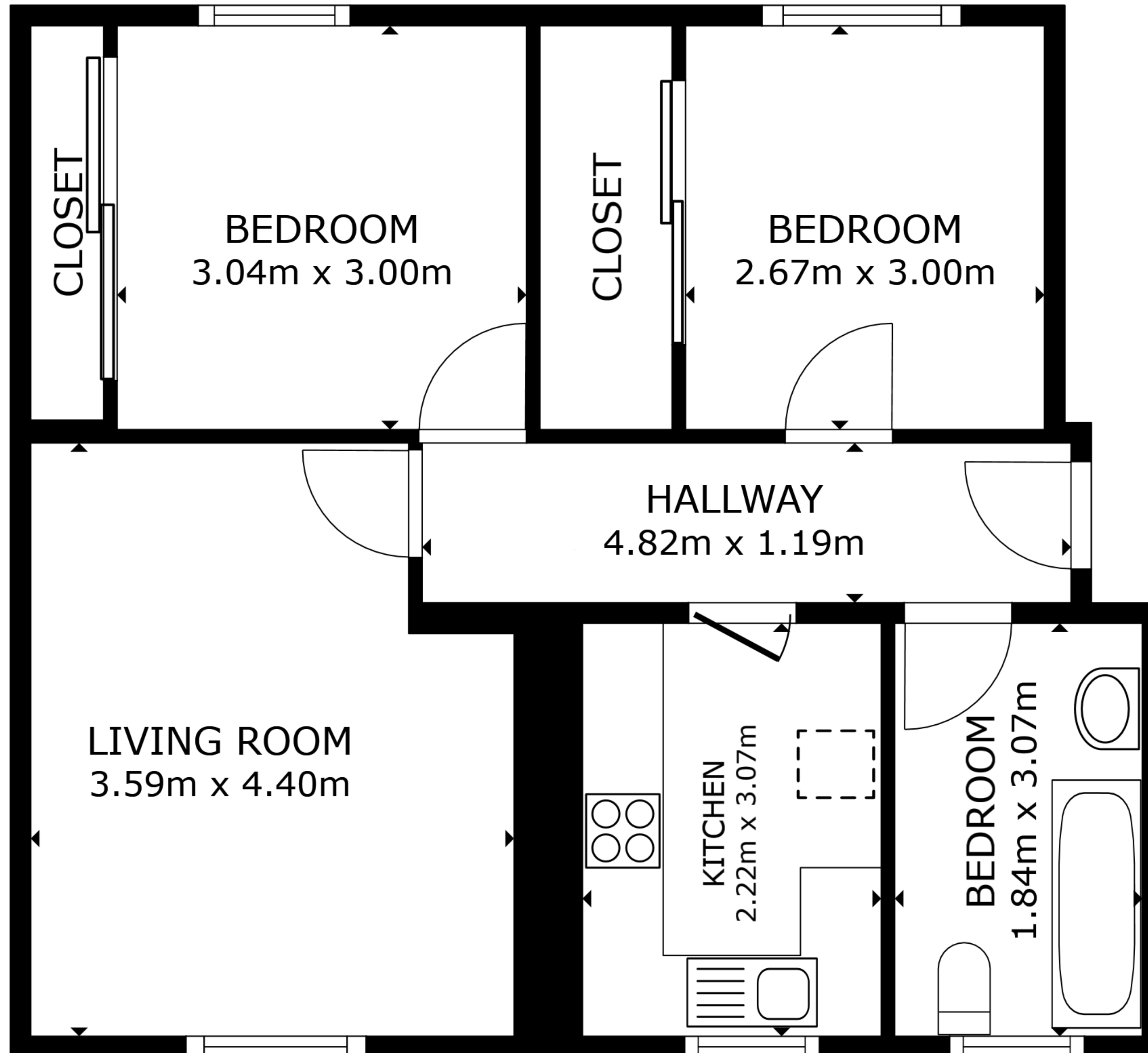
FLOOR PLAN
