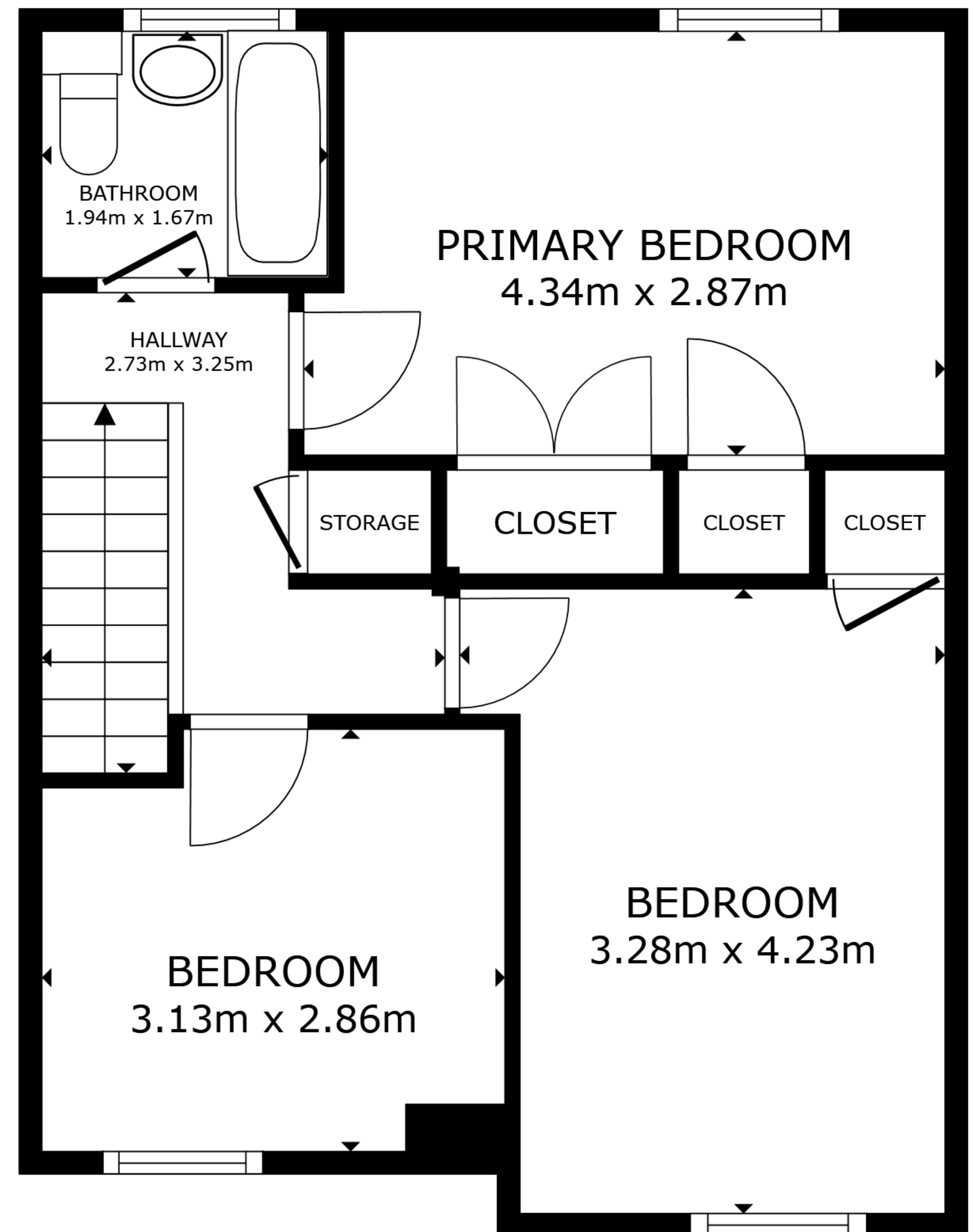
FLOOR 2
