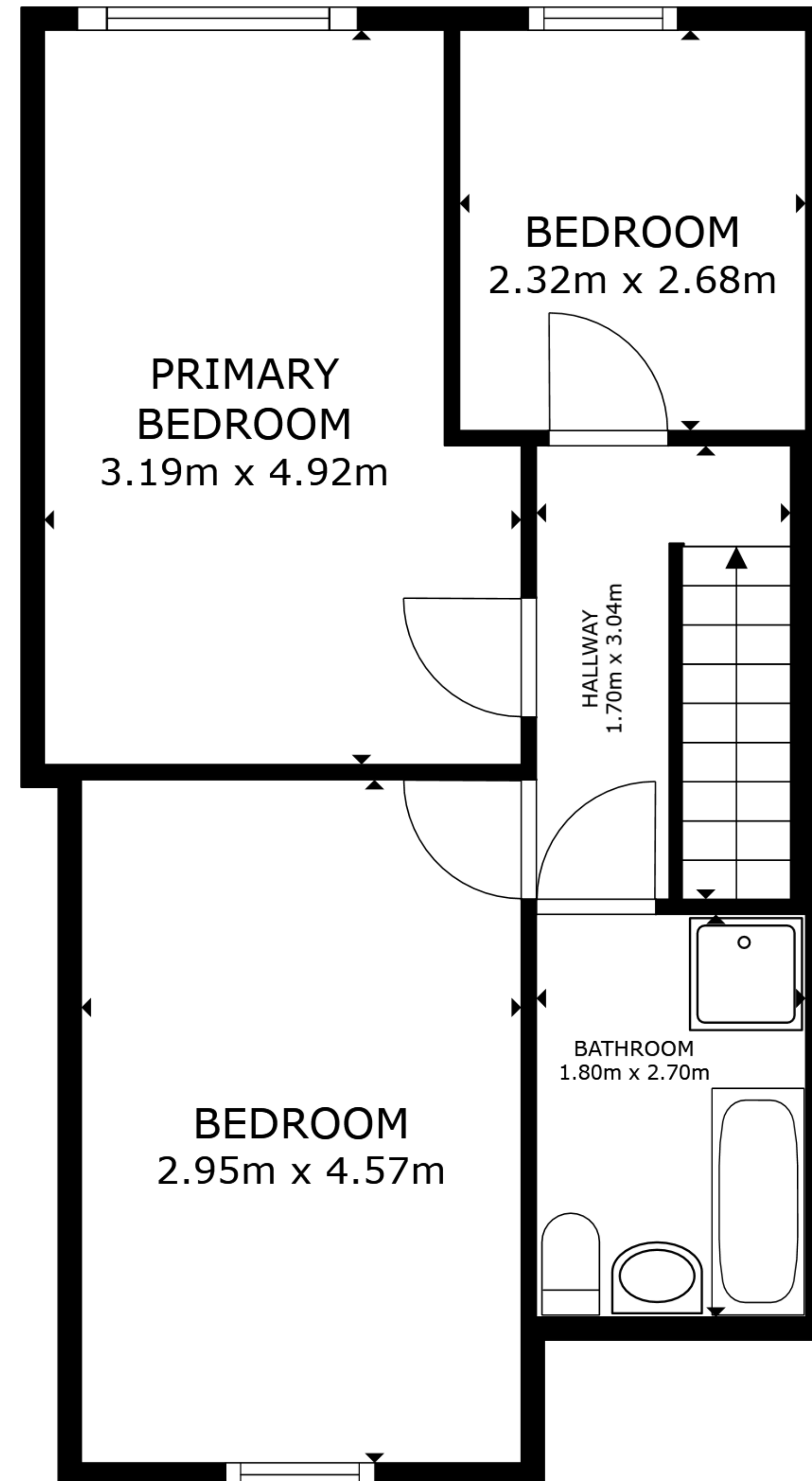
FLOOR 2
