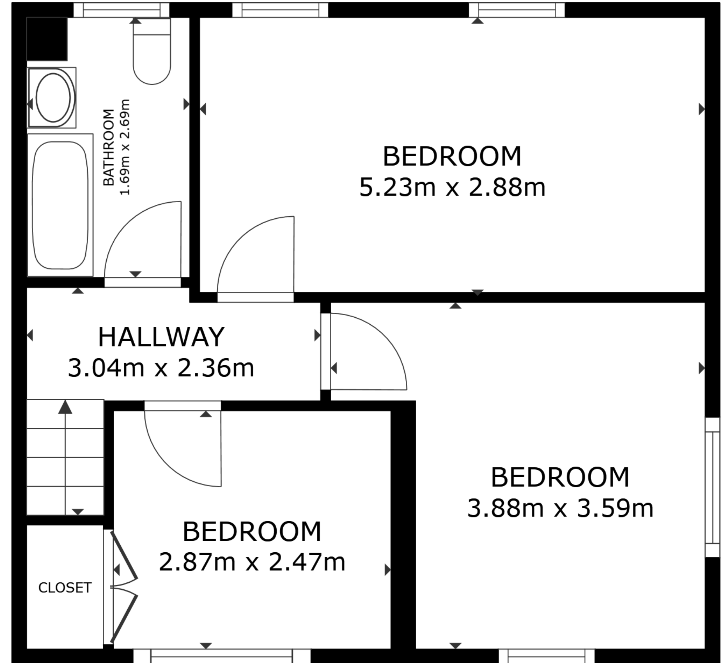
FLOOR 2
