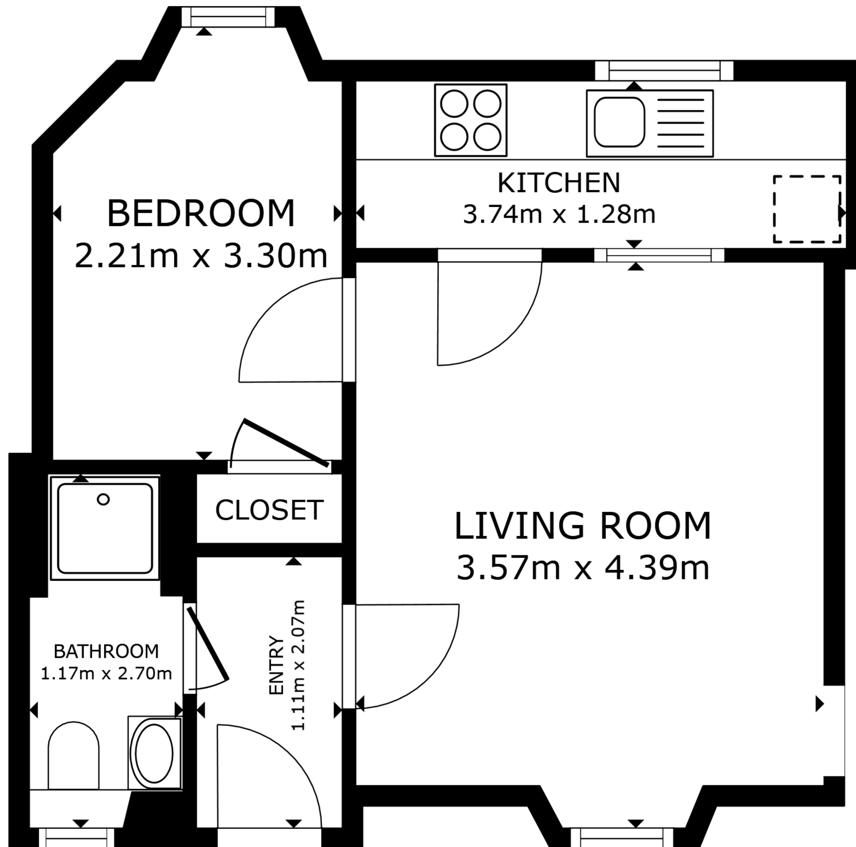
FLOOR PLAN
