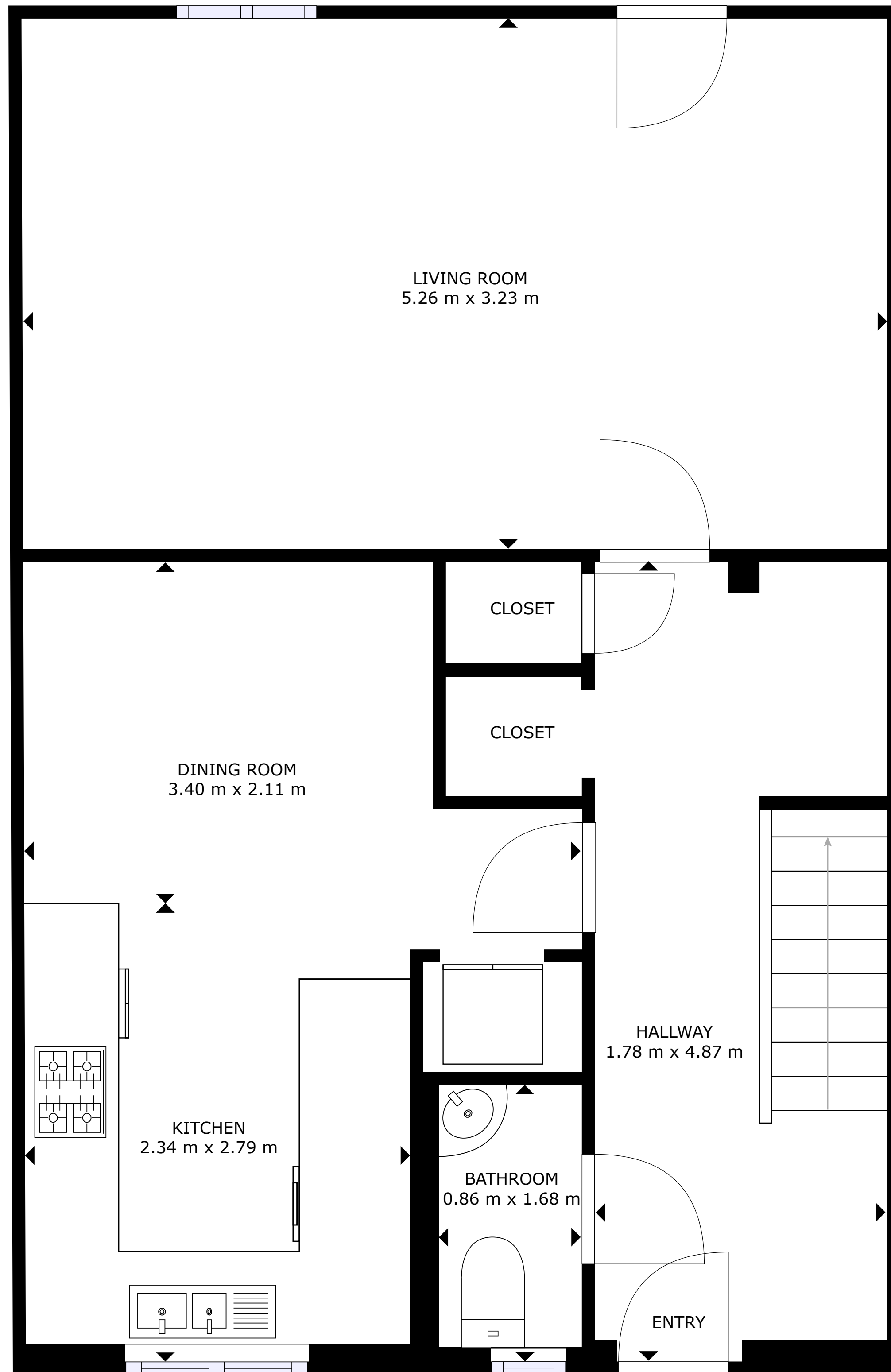
FLOOR 1
