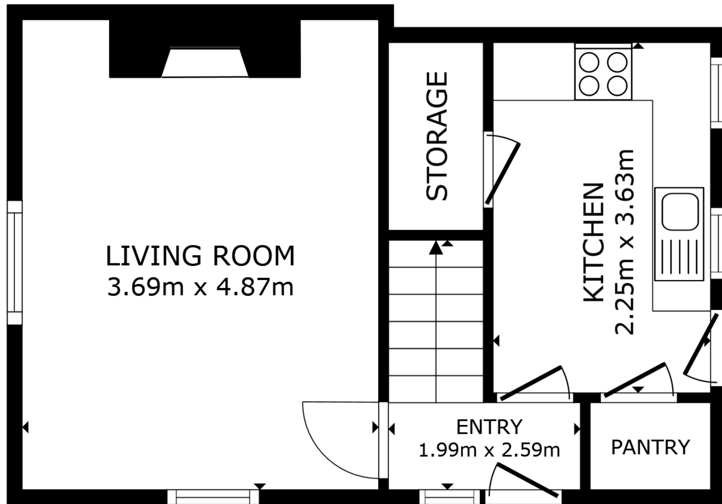
FLOOR 1
