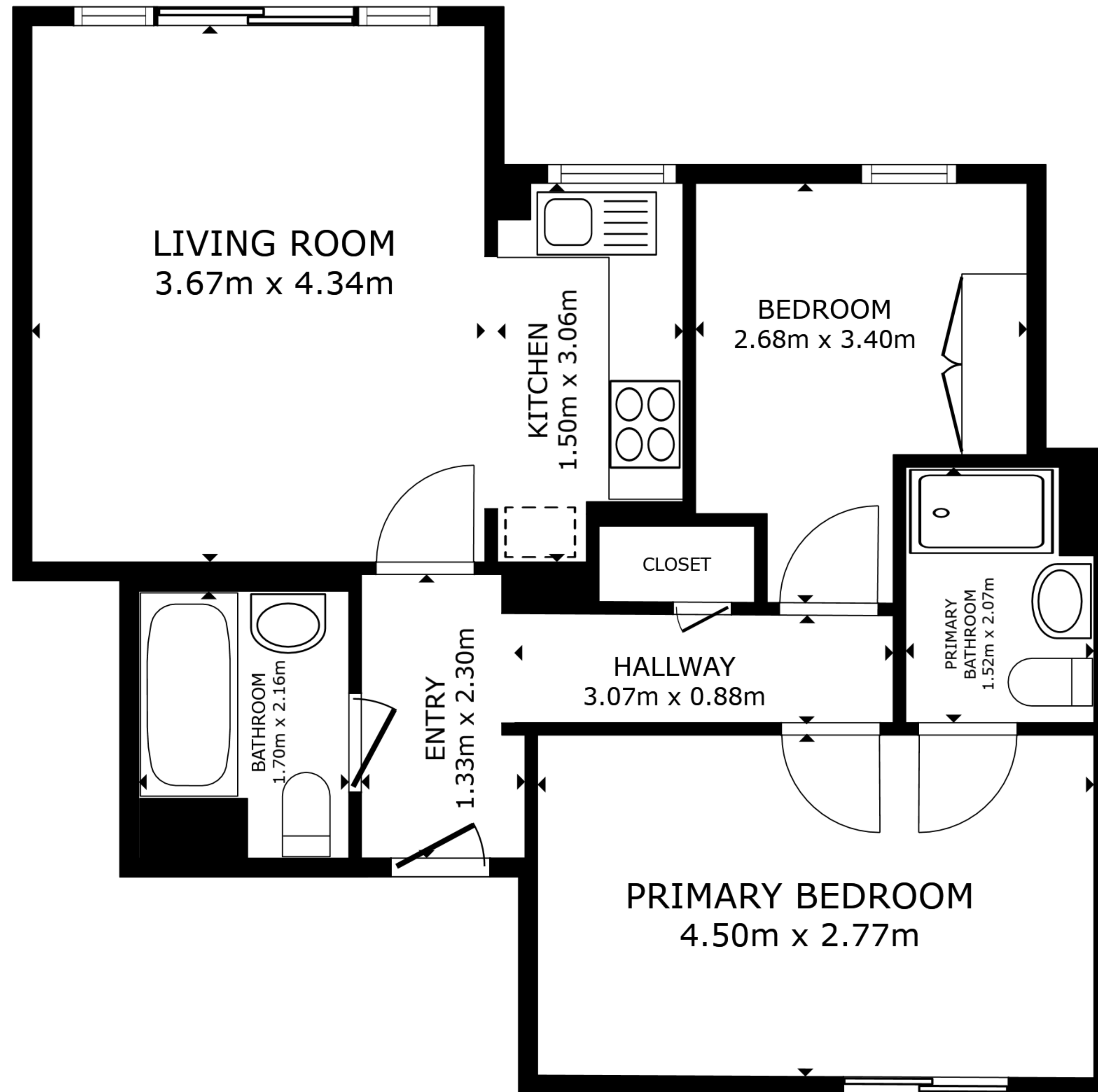
FLOOR PLAN
