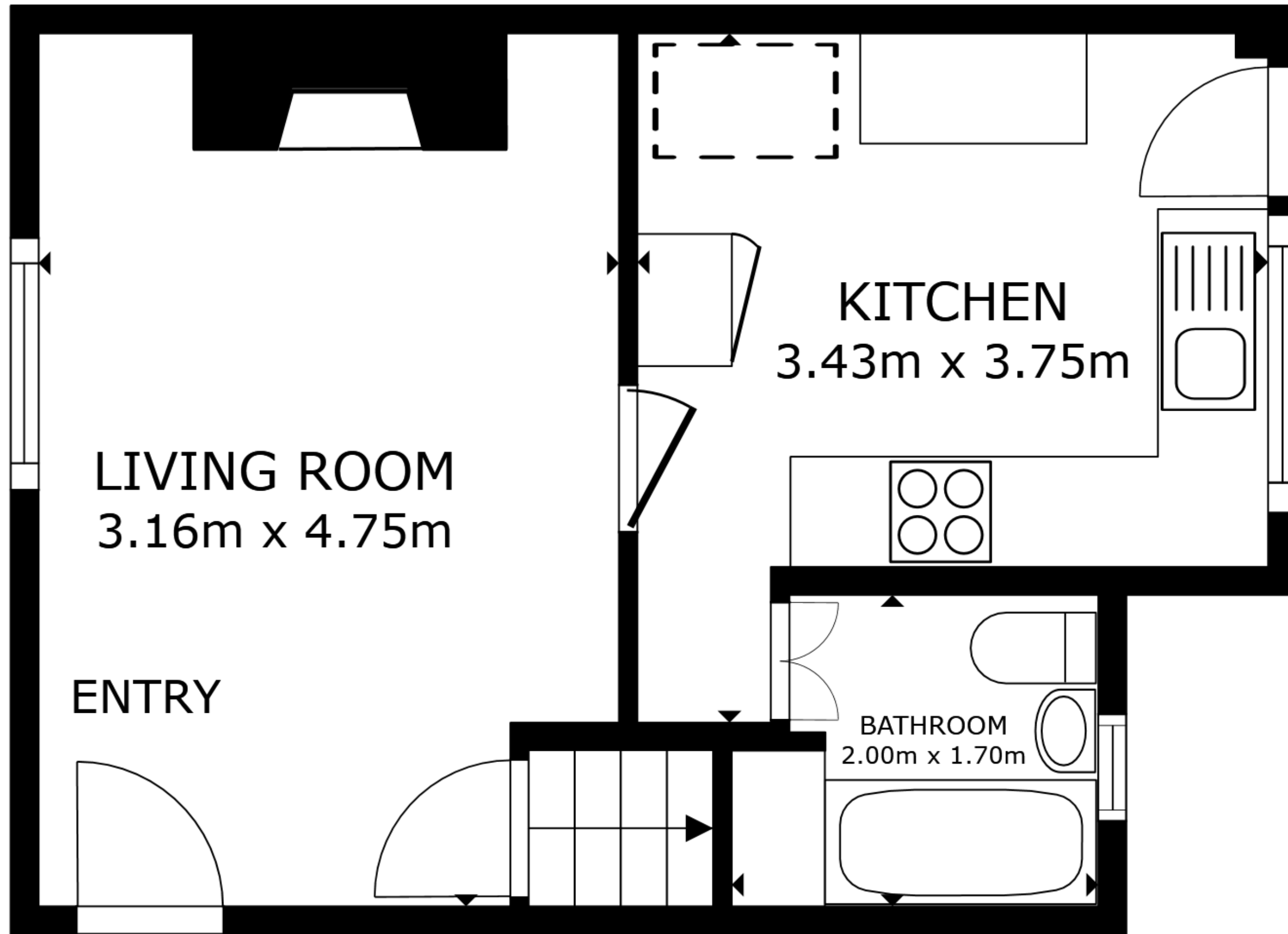
FLOOR 1
