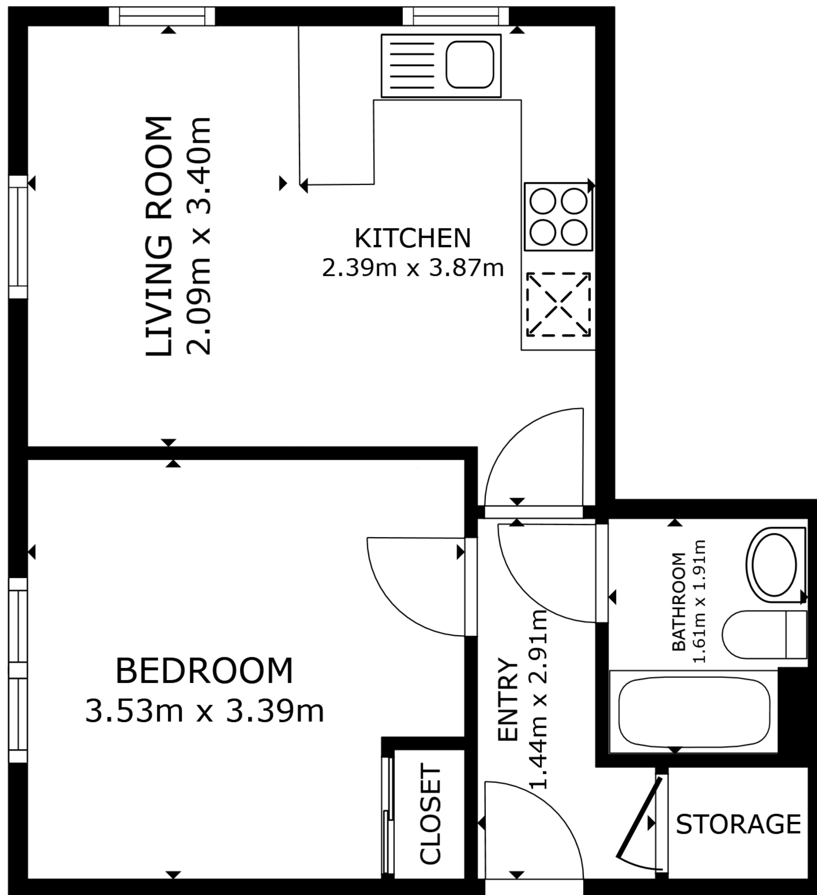
FLOOR PLAN
