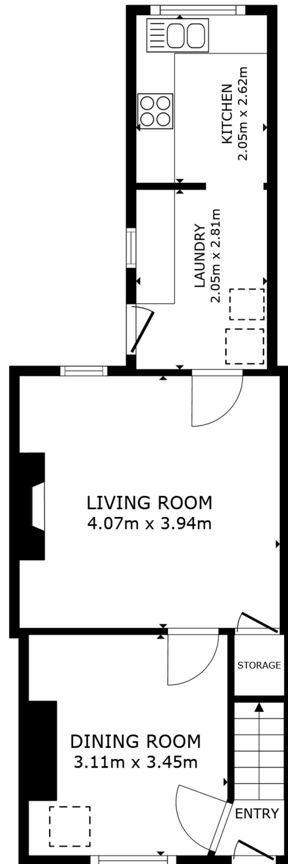
FLOOR 1
