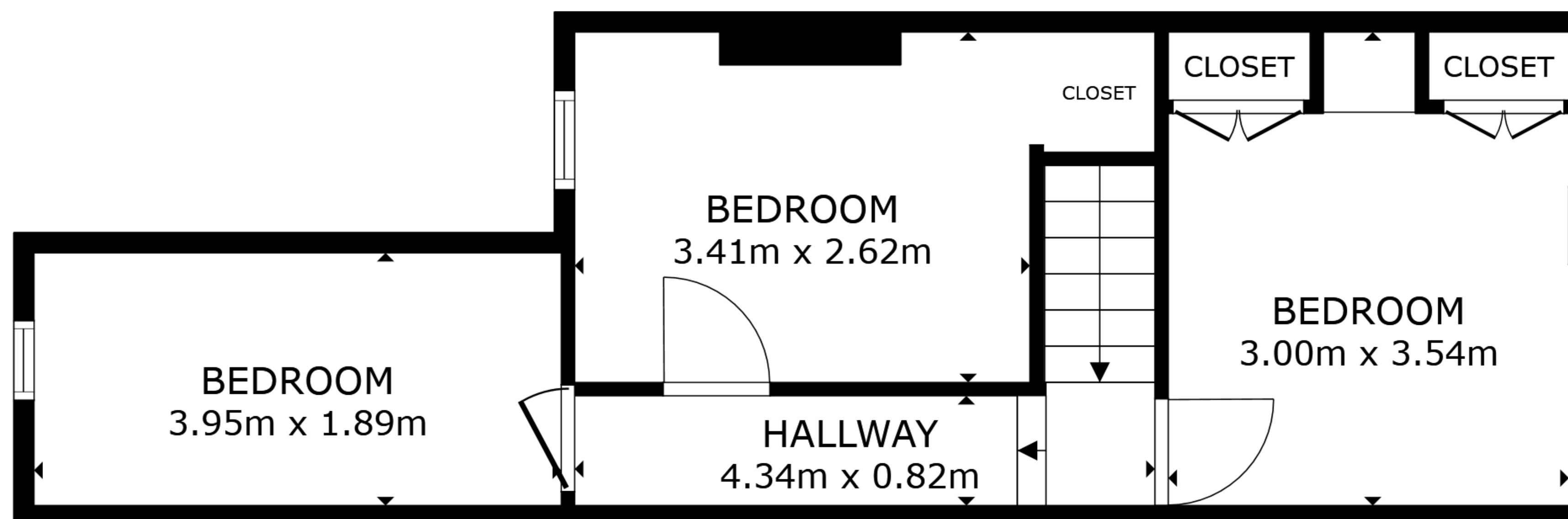
FLOOR 2
