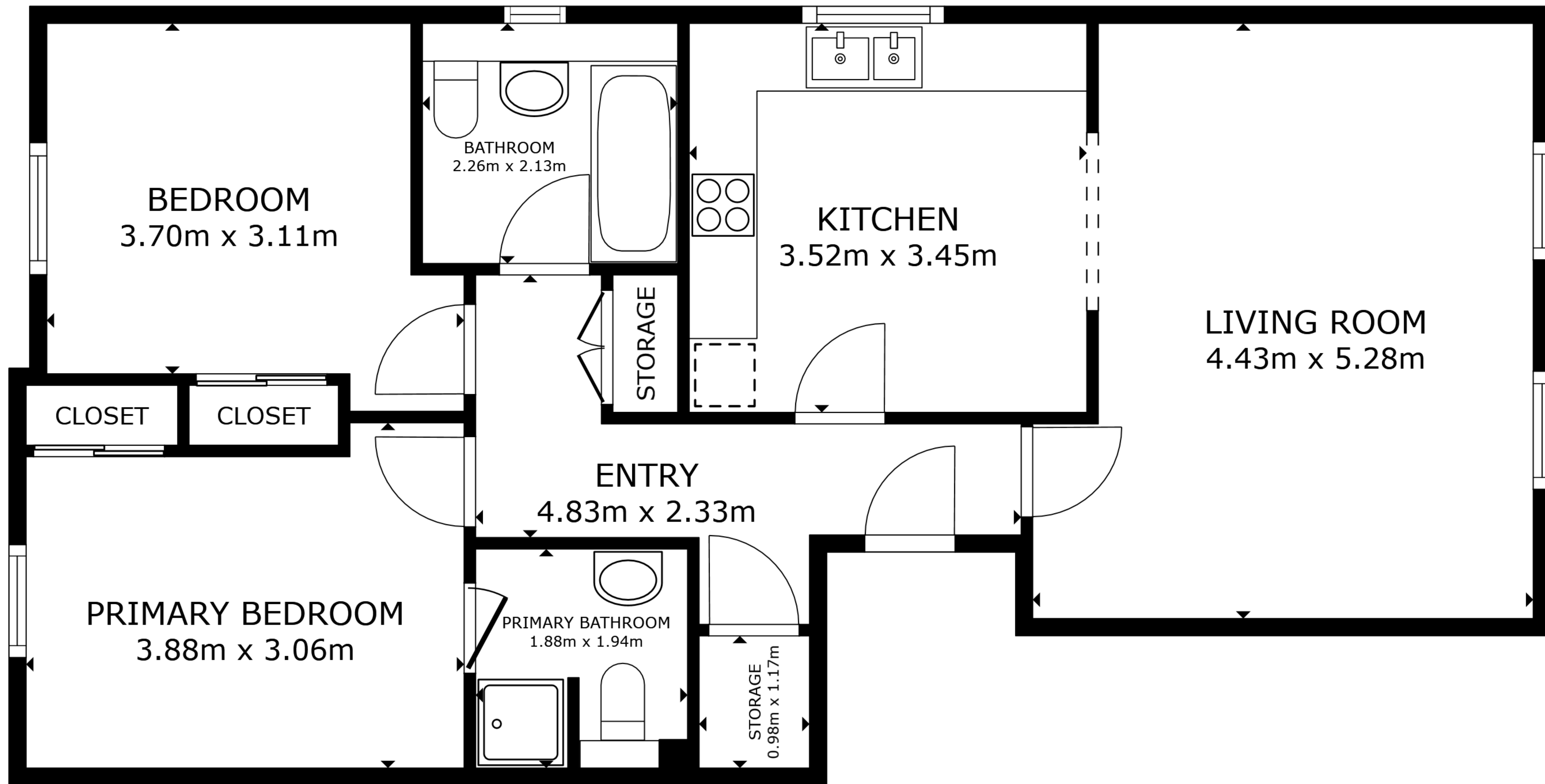
FLOOR PLAN
