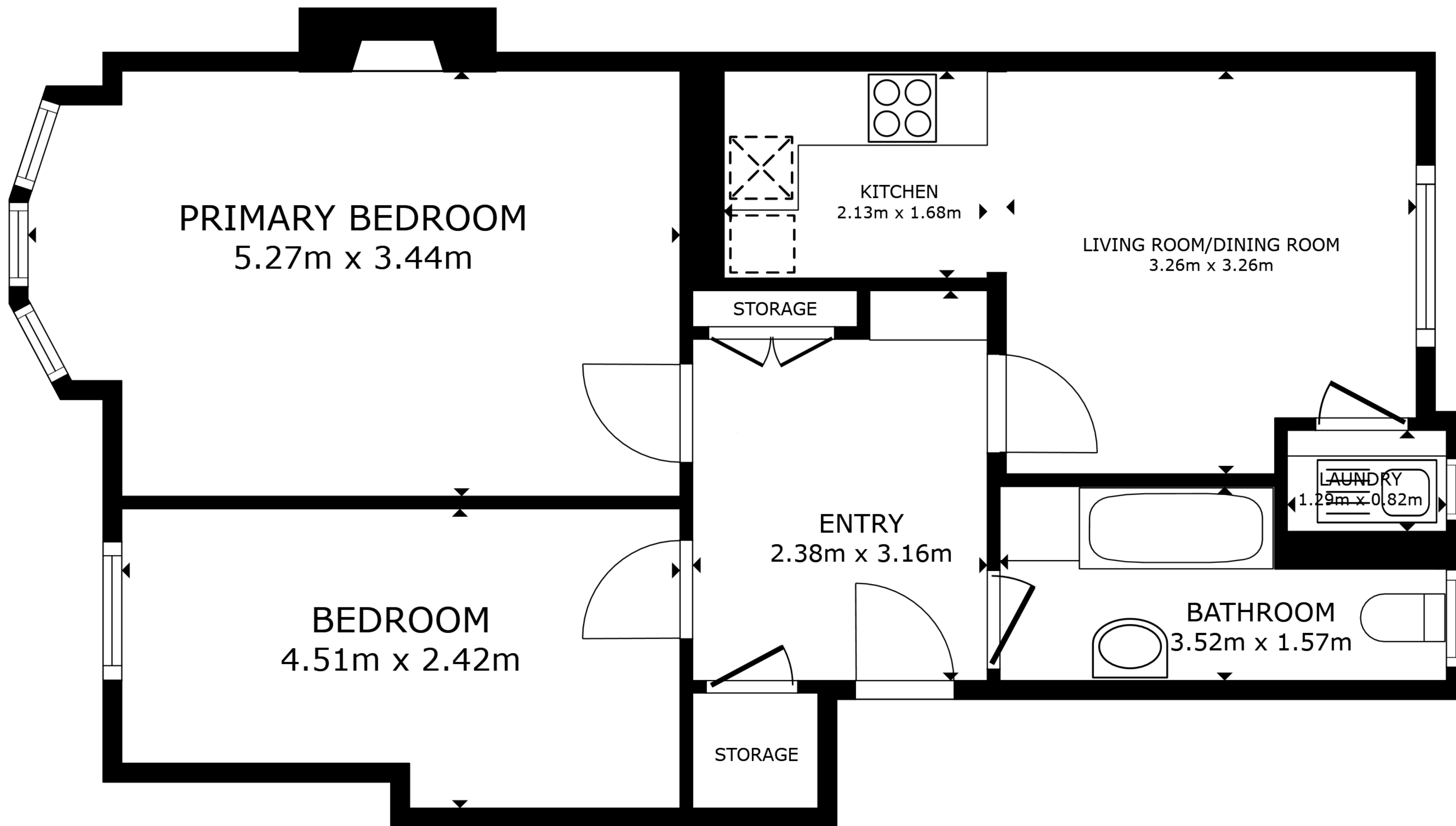
FLOOR PLAN
